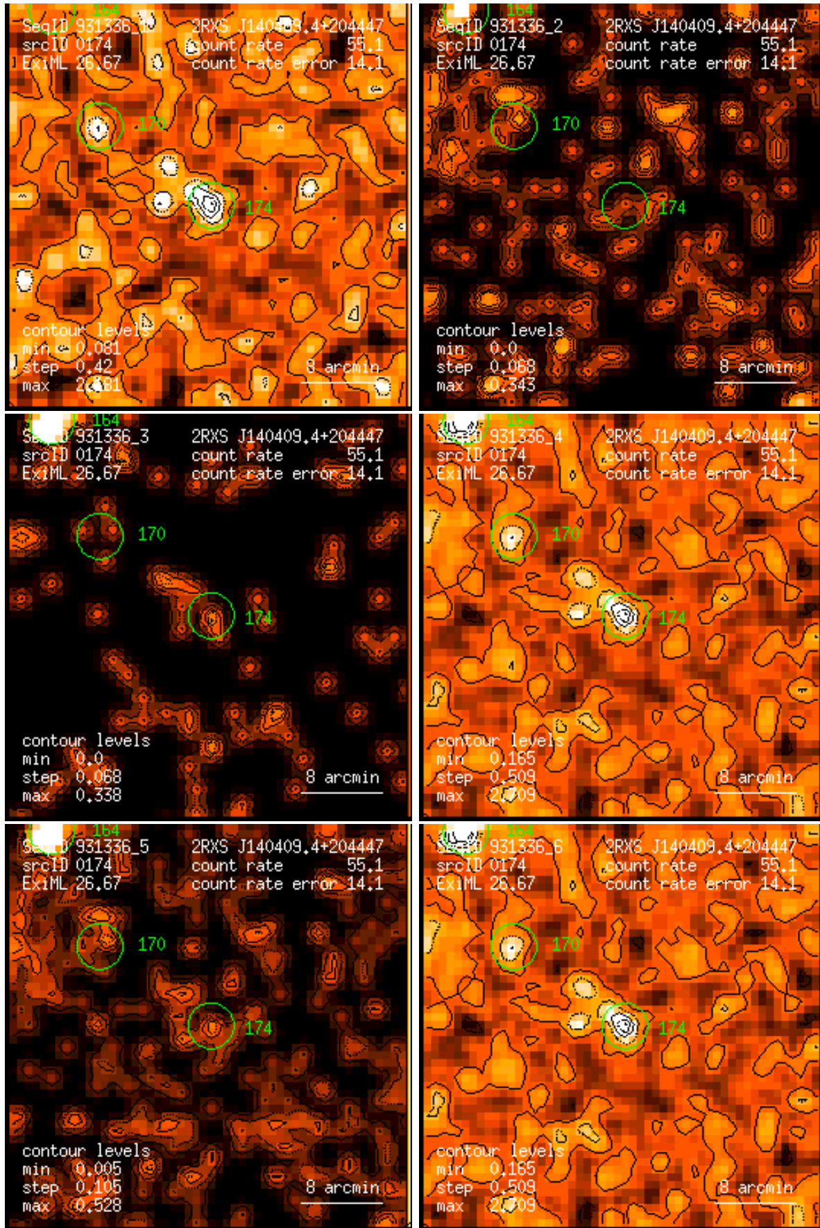
Figure 174: RASS 931336: detection 0174: band rate images, Gaussian filter: (1) PSPC channels 11 – 41, (2) 52 – 90, (3) 91 – 201, (4) 11 – 235, (5) 52 – 201, (6) 11 – 201. Broad band rates in counts/ks. Band rate contour levels in counts/ks/arcmin 2 .
