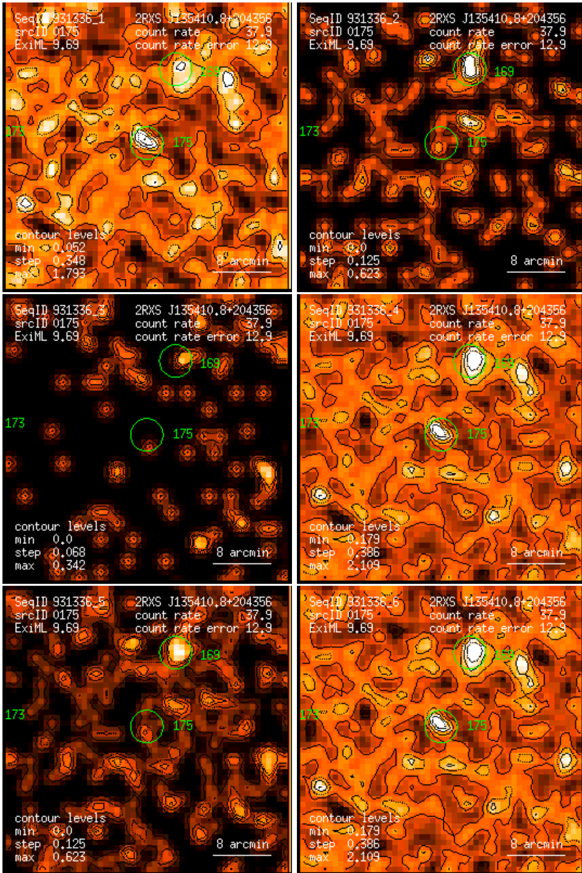
Figure 175: RASS 931336: detection 0175: band rate images, Gaussian filter: (1) PSPC channels 11 – 41, (2) 52 – 90, (3) 91 – 201, (4) 11 – 235, (5) 52 – 201, (6) 11 – 201. Broad band rates in counts/ks. Band rate contour levels in counts/ks/arcmin 2 .
