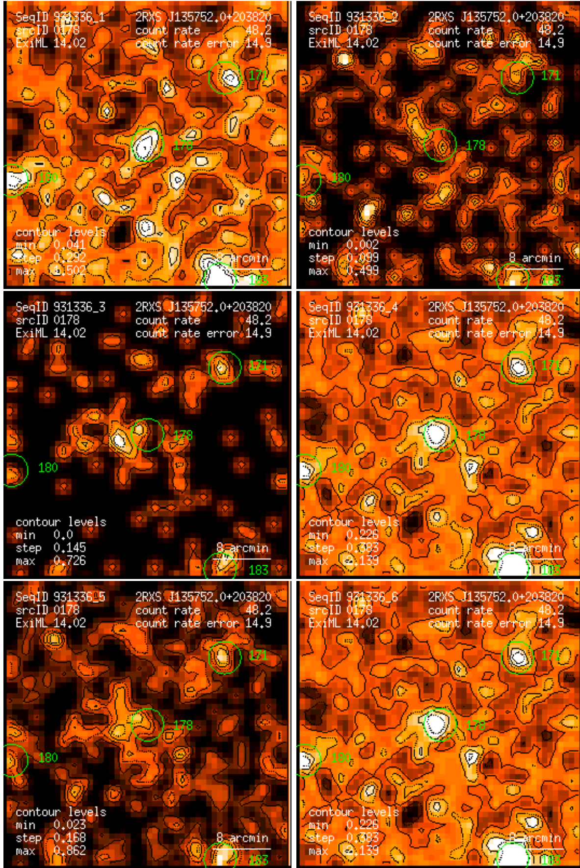
Figure 178: RASS 931336: detection 0178: band rate images, Gaussian filter: (1) PSPC channels 11 – 41, (2) 52 – 90, (3) 91 – 201, (4) 11 – 235, (5) 52 – 201, (6) 11 – 201. Broad band rates in counts/ks. Band rate contour levels in counts/ks/arcmin 2 .
