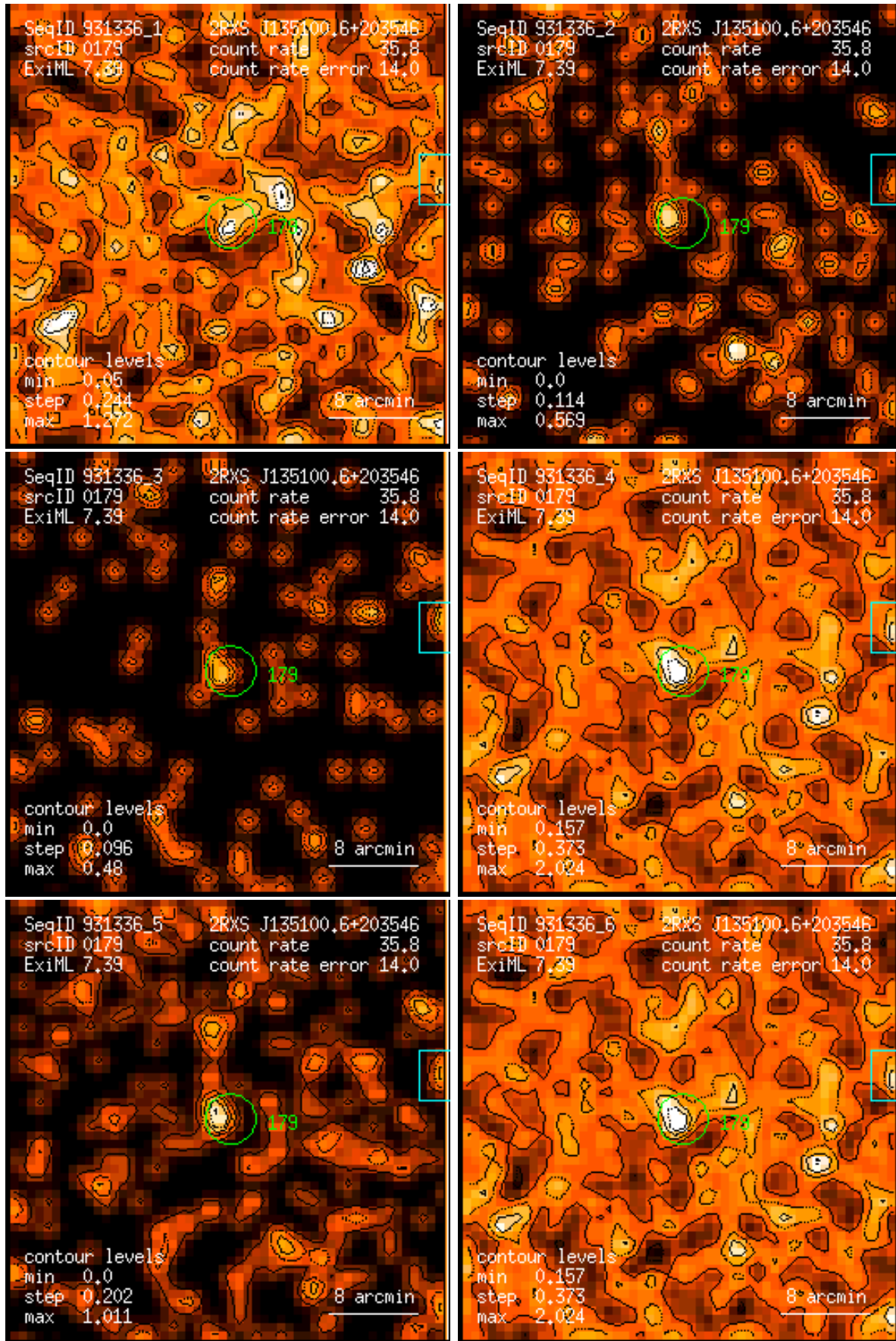
Figure 179: RASS 931336: detection 0179: band rate images, Gaussian filter: (1) PSPC channels 11 – 41, (2) 52 – 90, (3) 91 – 201, (4) 11 – 235, (5) 52 – 201, (6) 11 – 201. Broad band rates in counts/ks. Band rate contour levels in counts/ks/arcmin 2 .
