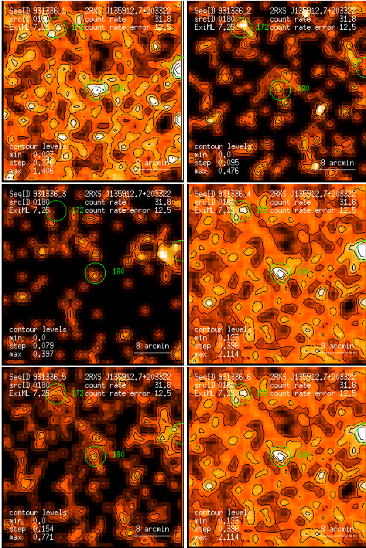
Figure 180: RASS 931336: detection 0180: band rate images, Gaussian filter: (1) PSPC channels 11 – 41, (2) 52 – 90, (3) 91 – 201, (4) 11 – 235, (5) 52 – 201, (6) 11 – 201. Broad band rates in counts/ks. Band rate contour levels in counts/ks/arcmin 2 .
