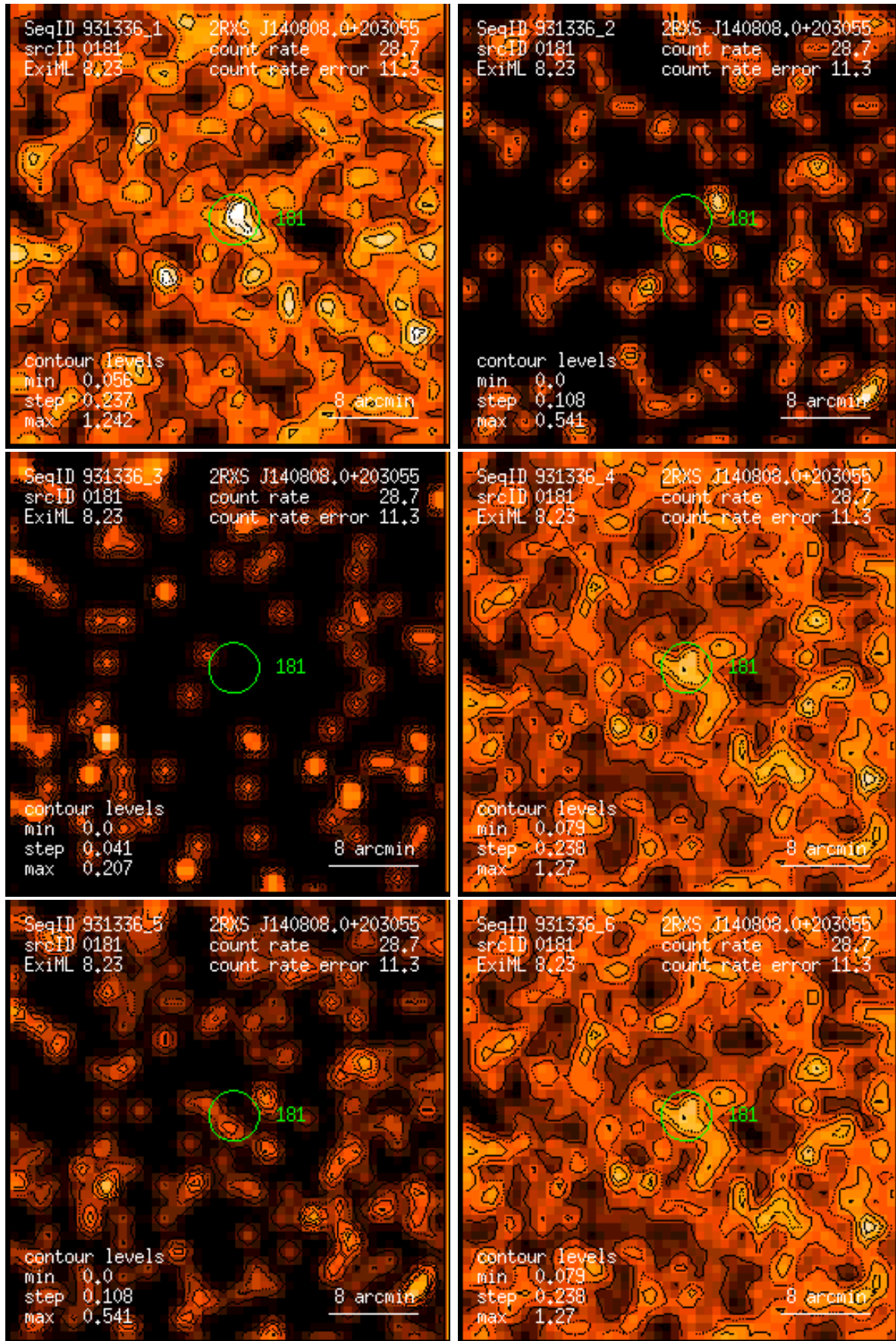
Figure 181: RASS 931336: detection 0181: band rate images, Gaussian filter: (1) PSPC channels 11 – 41, (2) 52 – 90, (3) 91 – 201, (4) 11 – 235, (5) 52 – 201, (6) 11 – 201. Broad band rates in counts/ks. Band rate contour levels in counts/ks/arcmin 2 .
