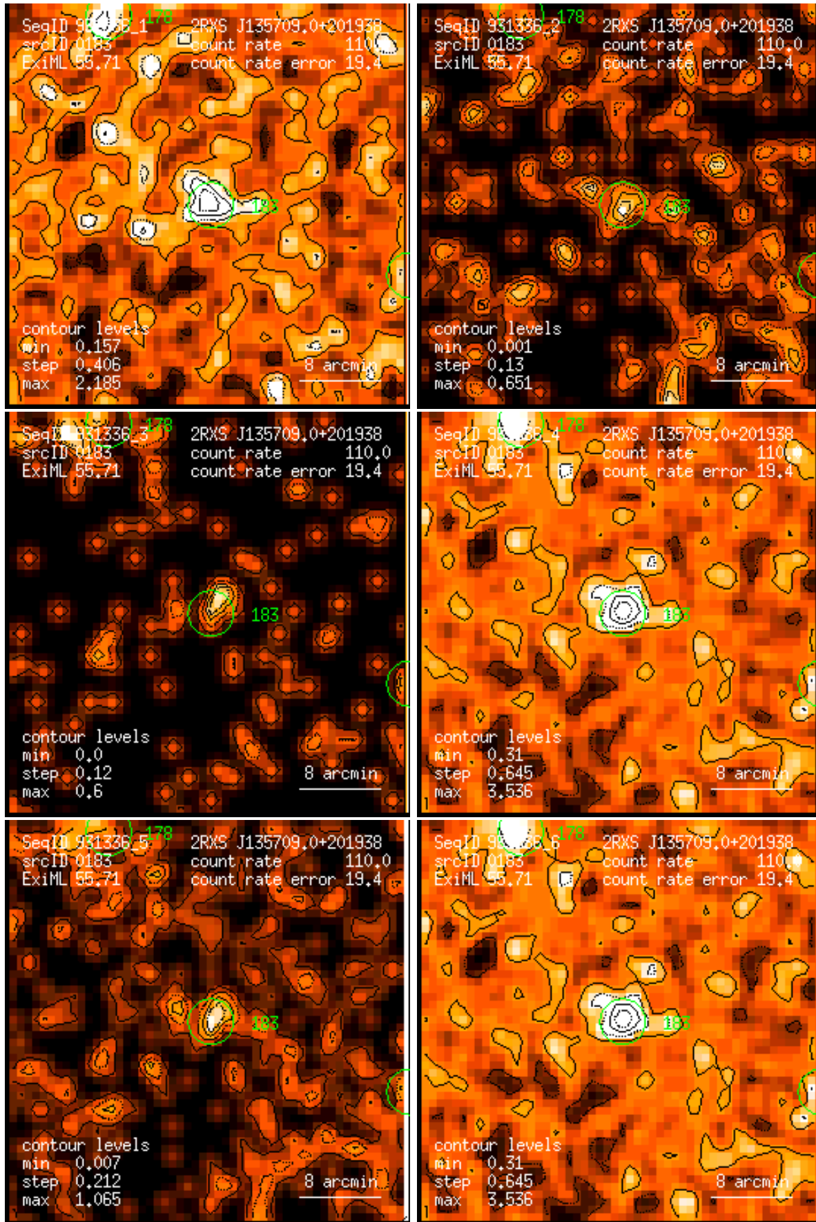
Figure 183: RASS 931336: detection 0183: band rate images, Gaussian filter: (1) PSPC channels 11 – 41, (2) 52 – 90, (3) 91 – 201, (4) 11 – 235, (5) 52 – 201, (6) 11 – 201. Broad band rates in counts/ks. Band rate contour levels in counts/ks/arcmin 2 .
