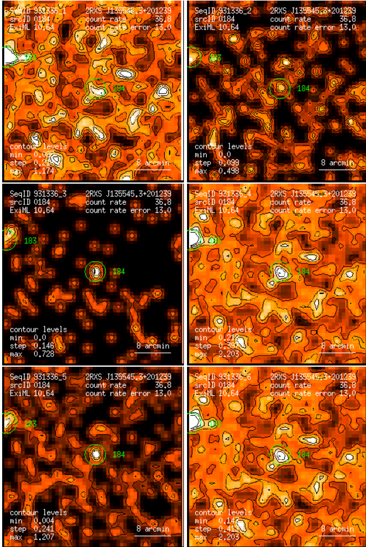
Figure 184: RASS 931336: detection 0184: band rate images, Gaussian filter: (1) PSPC channels 11 – 41, (2) 52 – 90, (3) 91 – 201, (4) 11 – 235, (5) 52 – 201, (6) 11 – 201. Broad band rates in counts/ks. Band rate contour levels in counts/ks/arcmin 2 .
