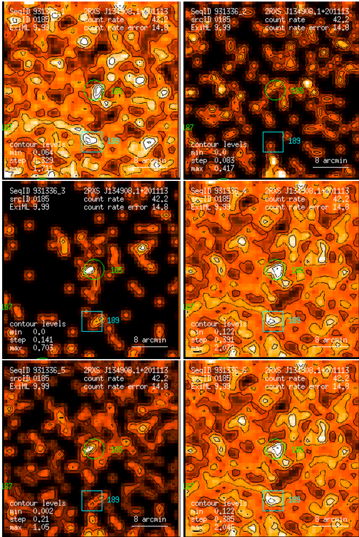
Figure 185: RASS 931336: detection 0185: band rate images, Gaussian filter: (1) PSPC channels 11 – 41, (2) 52 – 90, (3) 91 – 201, (4) 11 – 235, (5) 52 – 201, (6) 11 – 201. Broad band rates in counts/ks. Band rate contour levels in counts/ks/arcmin 2 .
