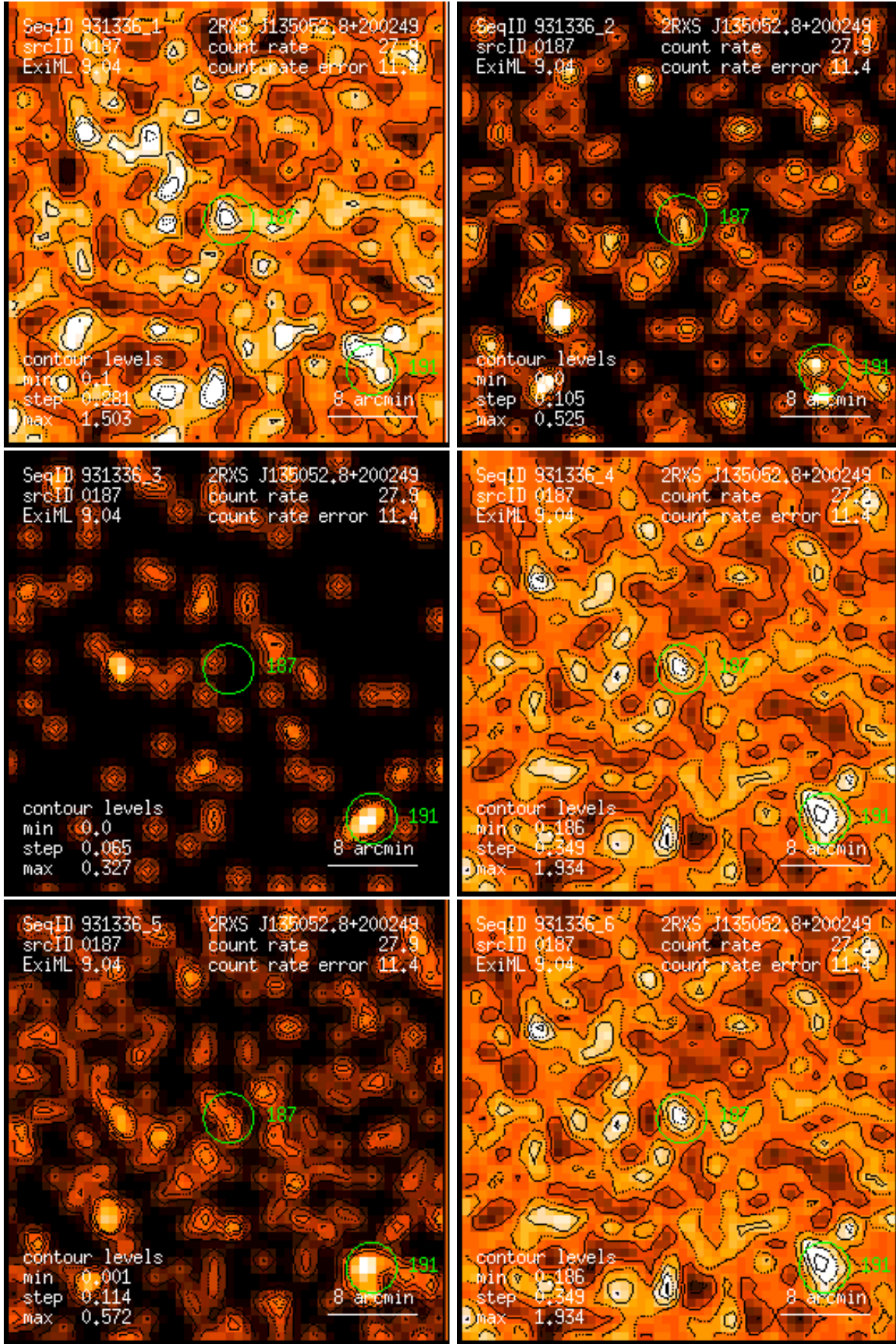
Figure 187: RASS 931336: detection 0187: band rate images, Gaussian filter: (1) PSPC channels 11 – 41, (2) 52 – 90, (3) 91 – 201, (4) 11 – 235, (5) 52 – 201, (6) 11 – 201. Broad band rates in counts/ks. Band rate contour levels in counts/ks/arcmin 2 .
