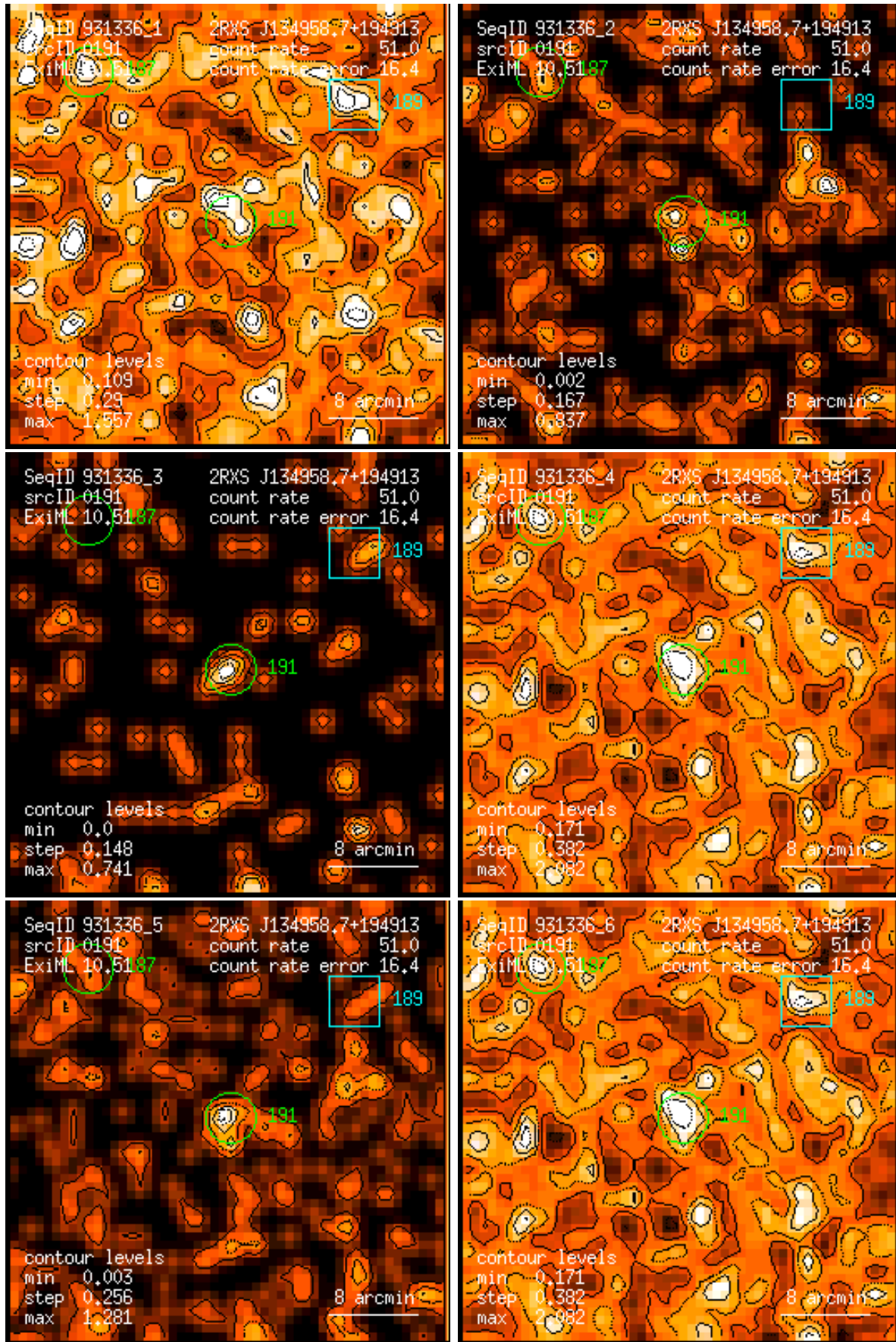
Figure 191: RASS 931336: detection 0191: band rate images, Gaussian filter: (1) PSPC channels 11 – 41, (2) 52 – 90, (3) 91 – 201, (4) 11 – 235, (5) 52 – 201, (6) 11 – 201. Broad band rates in counts/ks. Band rate contour levels in counts/ks/arcmin 2 .
