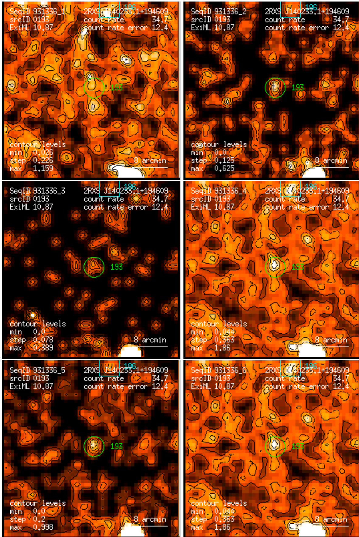
Figure 193: RASS 931336: detection 0193: band rate images, Gaussian filter: (1) PSPC channels 11 – 41, (2) 52 – 90, (3) 91 – 201, (4) 11 – 235, (5) 52 – 201, (6) 11 – 201. Broad band rates in counts/ks. Band rate contour levels in counts/ks/arcmin 2 .
