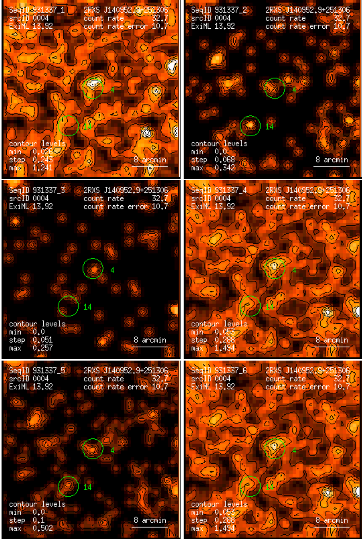
Figure 4: RASS 931337: detection 0004: band rate images, Gaussian filter: (1) PSPC channels 11 – 41, (2) 52 – 90, (3) 91 – 201, (4) 11 – 235, (5) 52 – 201, (6) 11 – 201. Broad band rates in counts/ks. Band rate contour levels in counts/ks/arcmin 2 .
