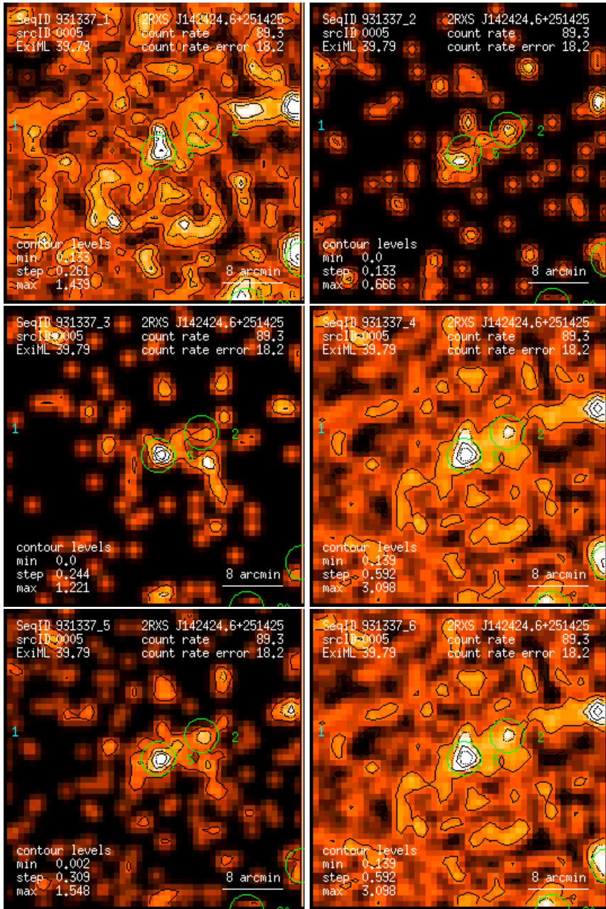
Figure 5: RASS 931337: detection 0005: band rate images, Gaussian filter: (1) PSPC channels 11 – 41, (2) 52 – 90, (3) 91 – 201, (4) 11 – 235, (5) 52 – 201, (6) 11 – 201. Broad band rates in counts/ks. Band rate contour levels in counts/ks/arcmin 2 .
