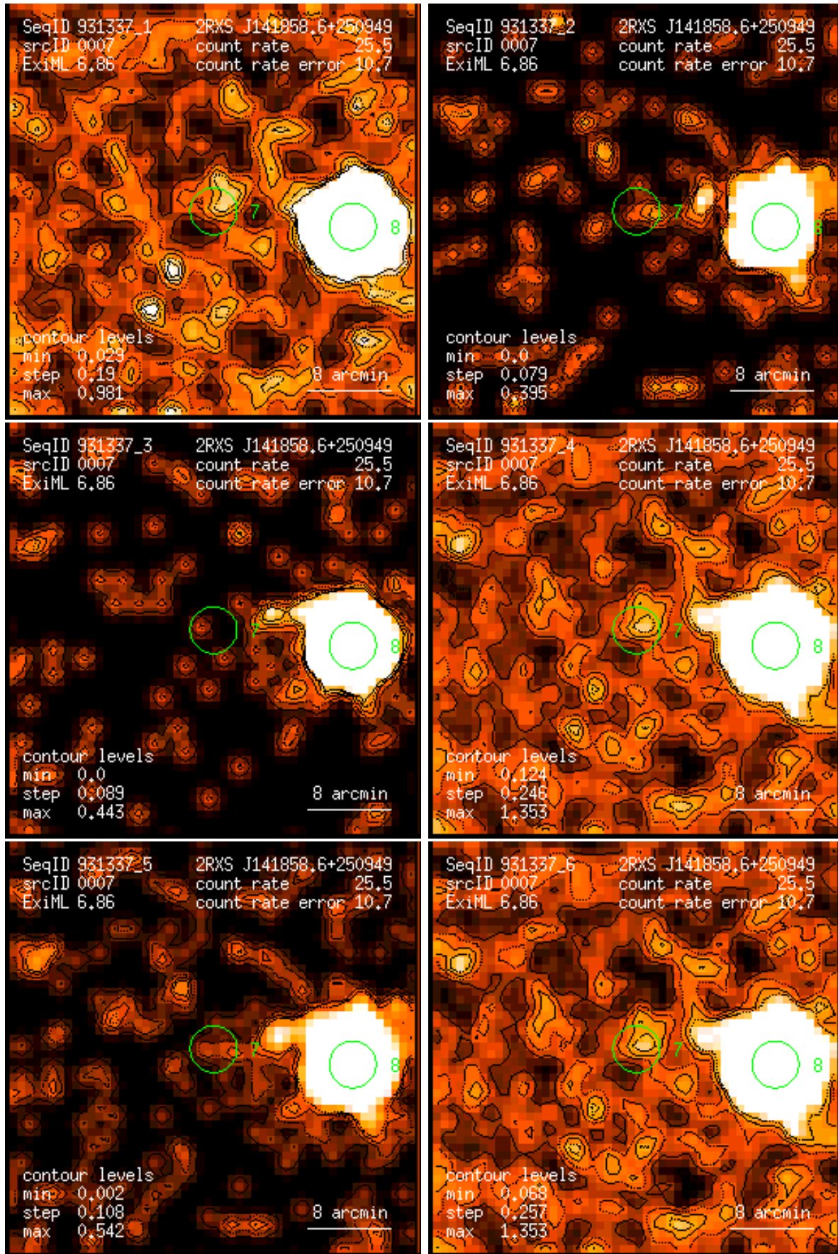
Figure 7: RASS 931337: detection 0007: band rate images, Gaussian filter: (1) PSPC channels 11 – 41, (2) 52 – 90, (3) 91 – 201, (4) 11 – 235, (5) 52 – 201, (6) 11 – 201. Broad band rates in counts/ks. Band rate contour levels in counts/ks/arcmin 2 .
