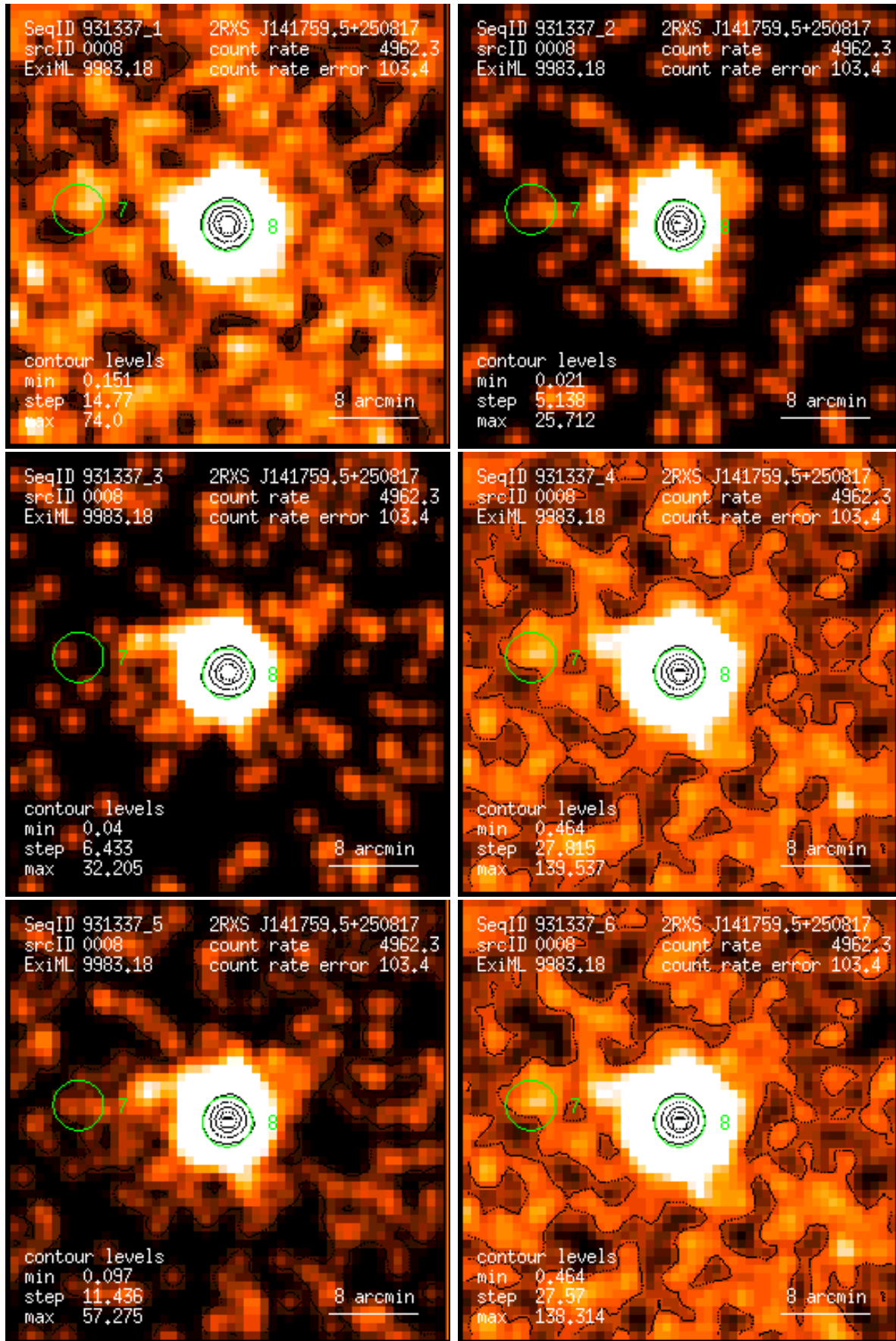
Figure 8: RASS 931337: detection 0008: band rate images, Gaussian filter: (1) PSPC channels 11 – 41, (2) 52 – 90, (3) 91 – 201, (4) 11 – 235, (5) 52 – 201, (6) 11 – 201. Broad band rates in counts/ks. Band rate contour levels in counts/ks/arcmin 2 .
