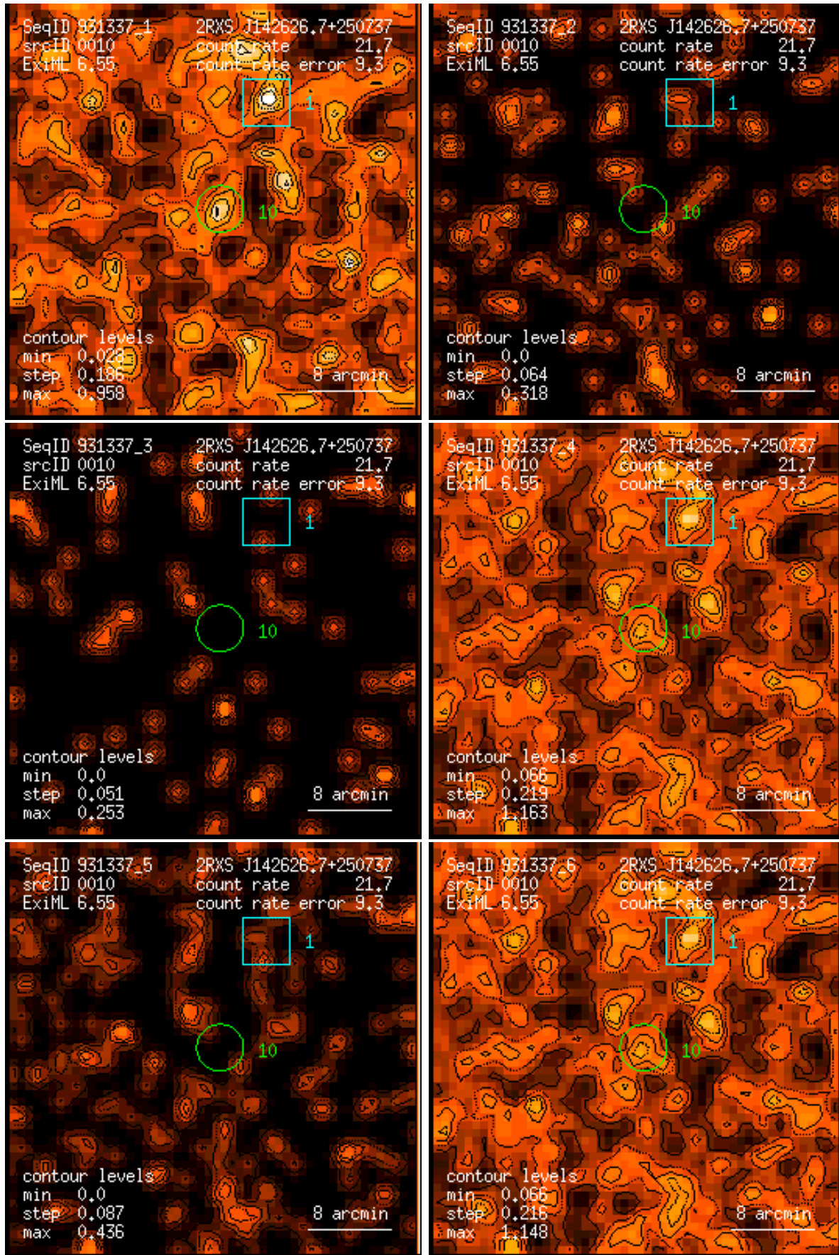
Figure 10: RASS 931337: detection 0010: band rate images, Gaussian filter: (1) PSPC channels 11 – 41, (2) 52 – 90, (3) 91 – 201, (4) 11 – 235, (5) 52 – 201, (6) 11 – 201. Broad band rates in counts/ks. Band rate contour levels in counts/ks/arcmin 2 .
