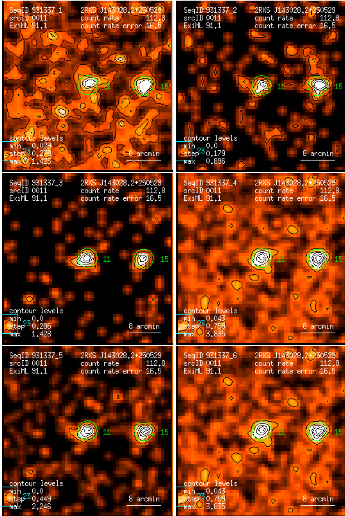
Figure 11: RASS 931337: detection 0011: band rate images, Gaussian filter: (1) PSPC channels 11 – 41, (2) 52 – 90, (3) 91 – 201, (4) 11 – 235, (5) 52 – 201, (6) 11 – 201. Broad band rates in counts/ks. Band rate contour levels in counts/ks/arcmin 2 .
