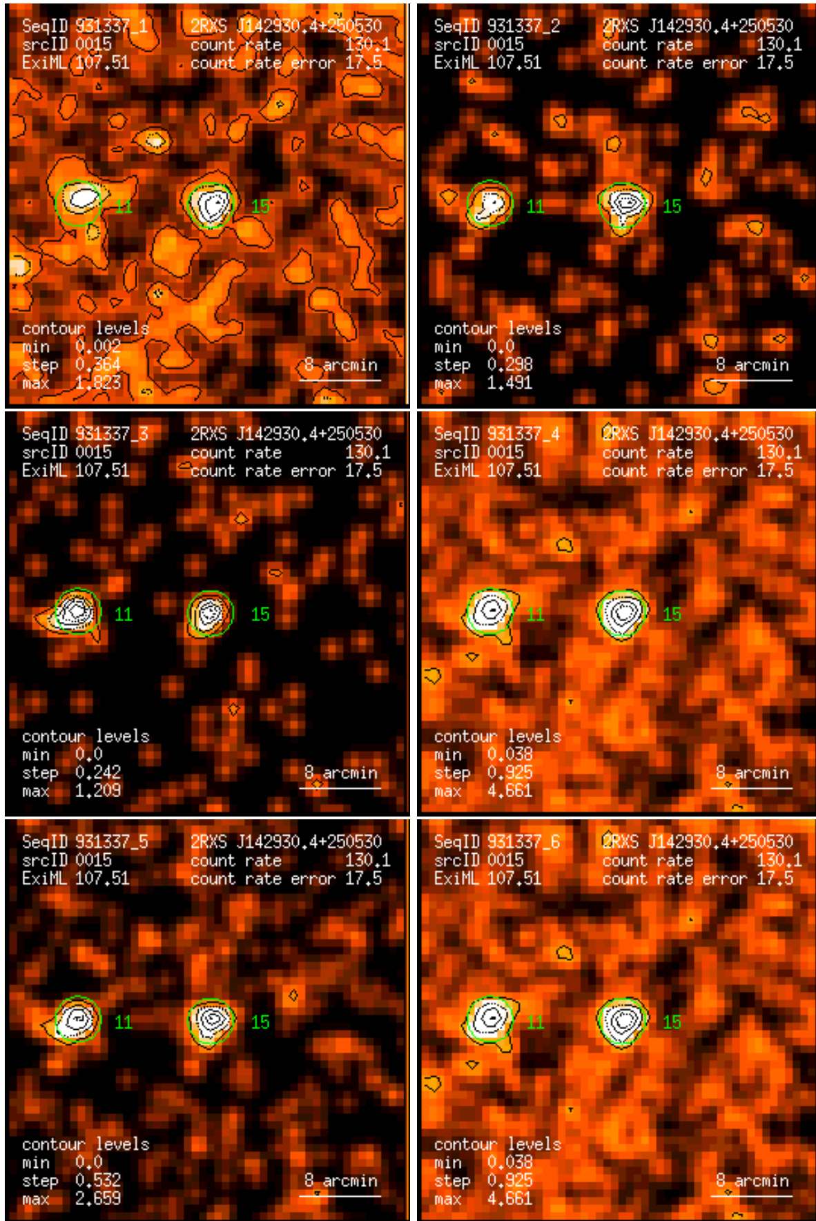
Figure 15: RASS 931337: detection 0015: band rate images, Gaussian filter: (1) PSPC channels 11 – 41, (2) 52 – 90, (3) 91 – 201, (4) 11 – 235, (5) 52 – 201, (6) 11 – 201. Broad band rates in counts/ks. Band rate contour levels in counts/ks/arcmin 2 .
