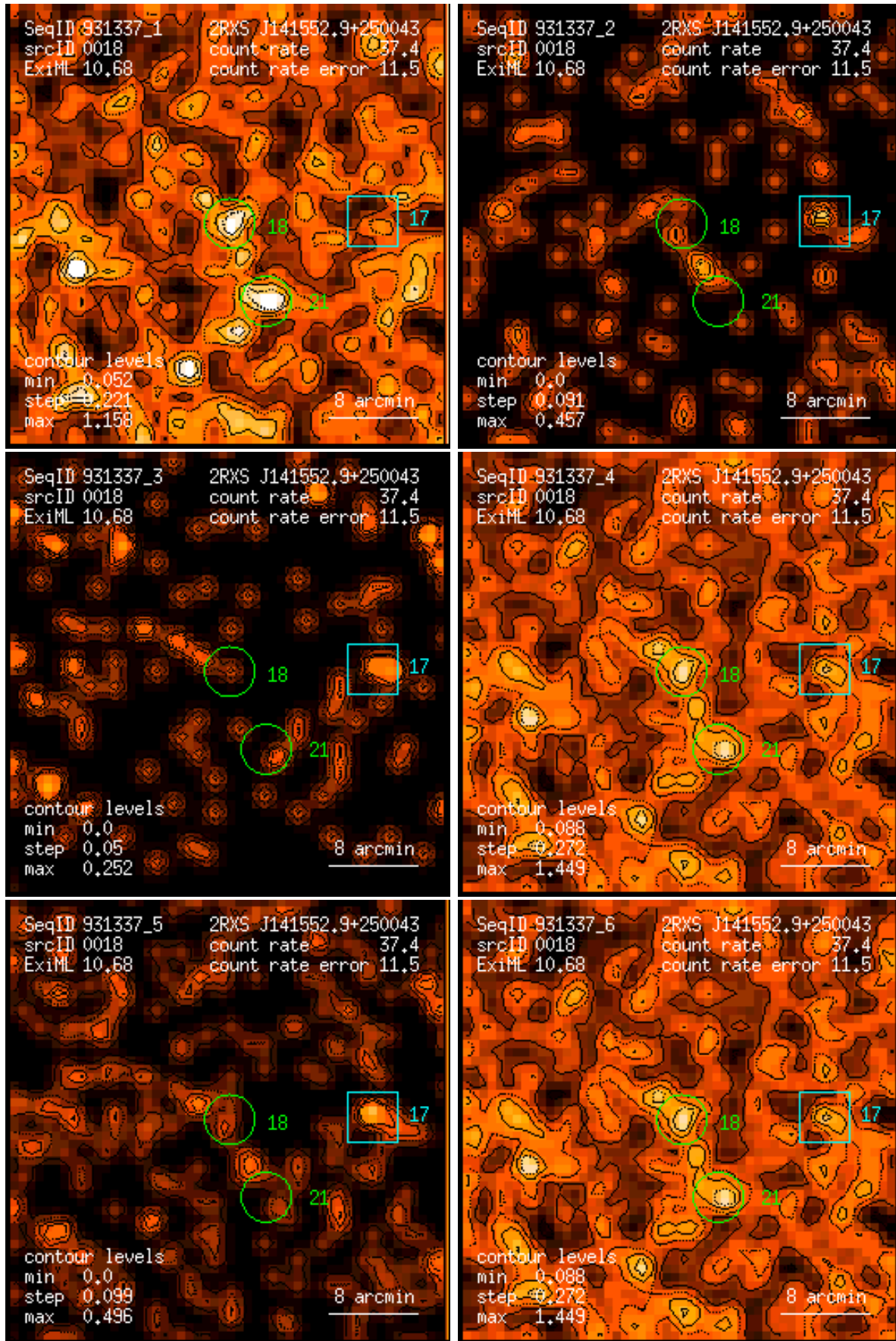
Figure 18: RASS 931337: detection 0018: band rate images, Gaussian filter: (1) PSPC channels 11 – 41, (2) 52 – 90, (3) 91 – 201, (4) 11 – 235, (5) 52 – 201, (6) 11 – 201. Broad band rates in counts/ks. Band rate contour levels in counts/ks/arcmin 2 .
