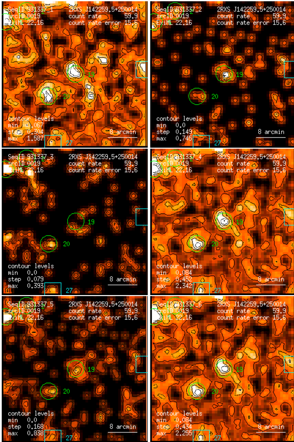
Figure 19: RASS 931337: detection 0019: band rate images, Gaussian filter: (1) PSPC channels 11 – 41, (2) 52 – 90, (3) 91 – 201, (4) 11 – 235, (5) 52 – 201, (6) 11 – 201. Broad band rates in counts/ks. Band rate contour levels in counts/ks/arcmin 2 .
