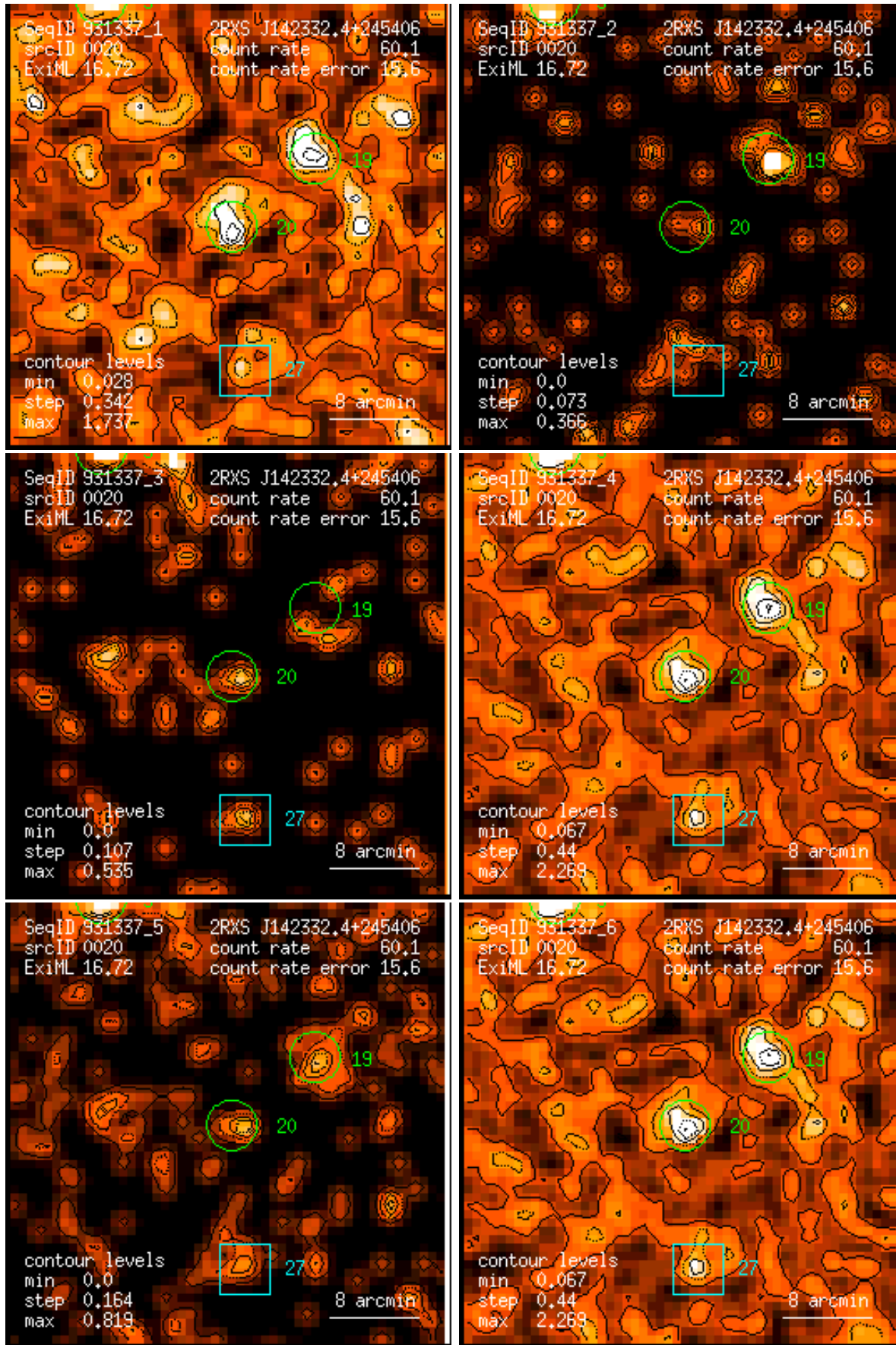
Figure 20: RASS 931337: detection 0020: band rate images, Gaussian filter: (1) PSPC channels 11 – 41, (2) 52 – 90, (3) 91 – 201, (4) 11 – 235, (5) 52 – 201, (6) 11 – 201. Broad band rates in counts/ks. Band rate contour levels in counts/ks/arcmin 2 .
