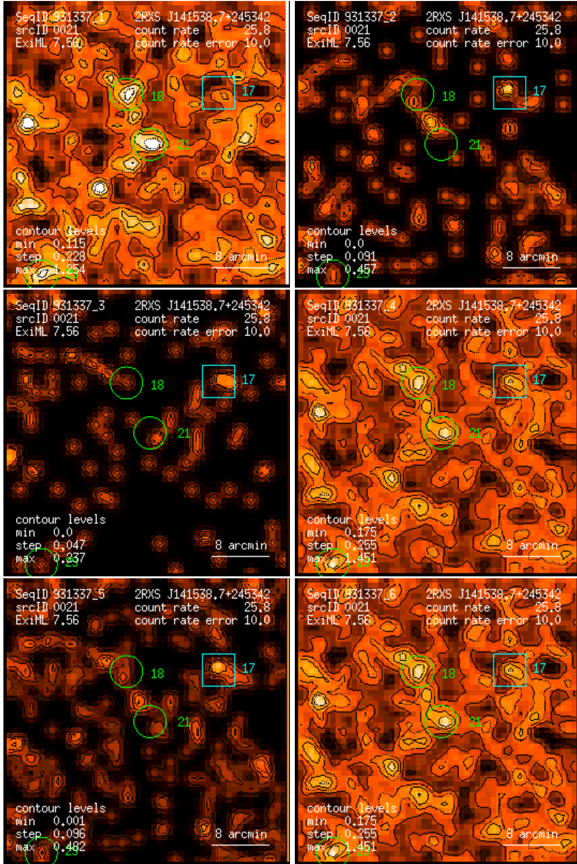
Figure 21: RASS 931337: detection 0021: band rate images, Gaussian filter: (1) PSPC channels 11 – 41, (2) 52 – 90, (3) 91 – 201, (4) 11 – 235, (5) 52 – 201, (6) 11 – 201. Broad band rates in counts/ks. Band rate contour levels in counts/ks/arcmin 2 .
