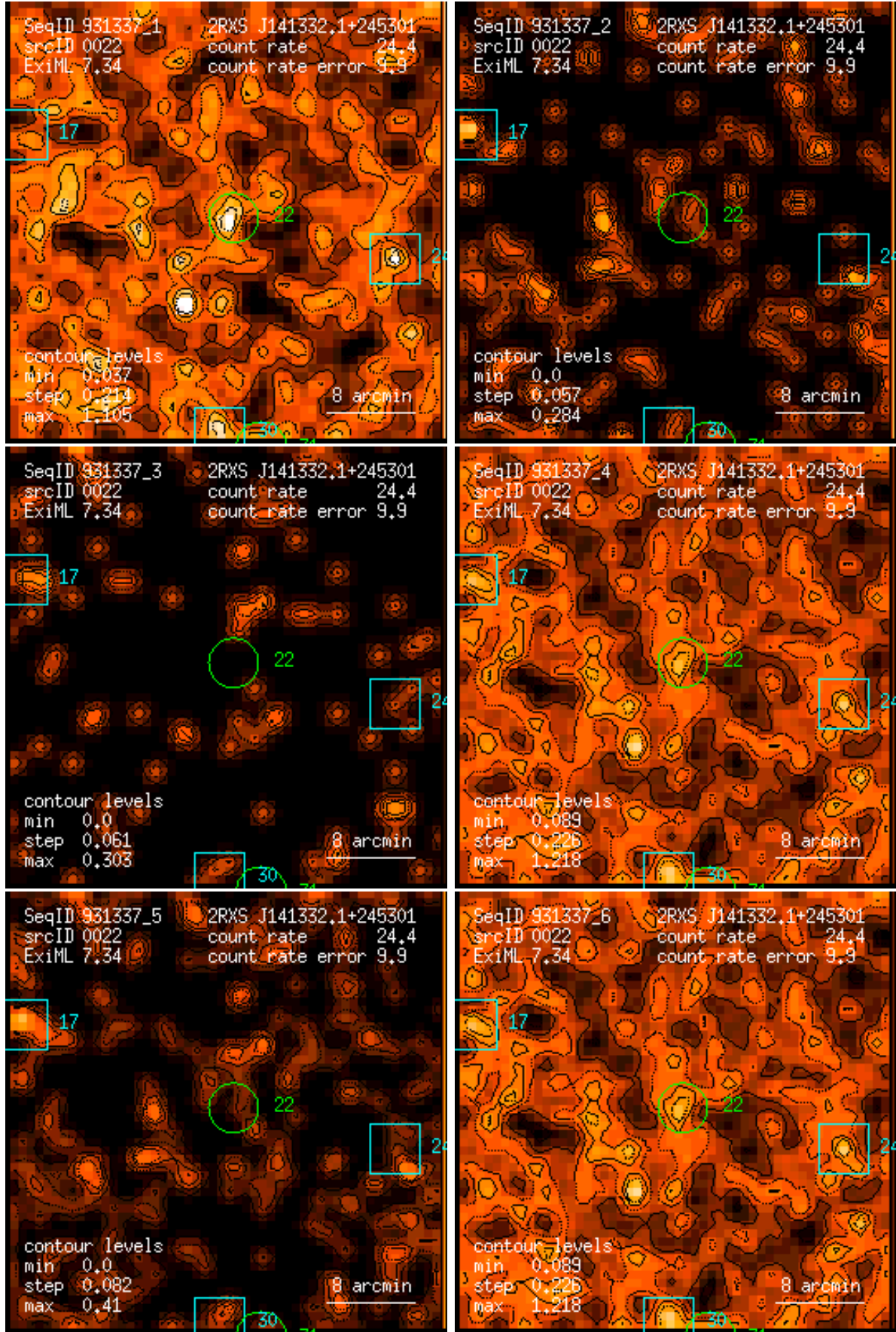
Figure 22: RASS 931337: detection 0022: band rate images, Gaussian filter: (1) PSPC channels 11 – 41, (2) 52 – 90, (3) 91 – 201, (4) 11 – 235, (5) 52 – 201, (6) 11 – 201. Broad band rates in counts/ks. Band rate contour levels in counts/ks/arcmin 2 .
