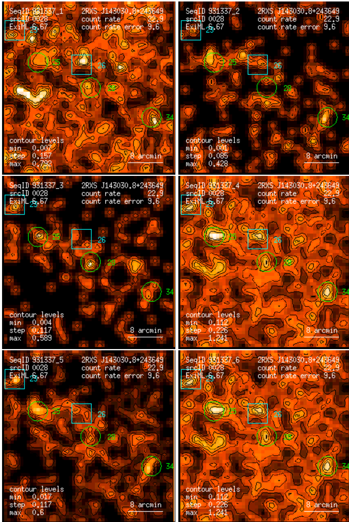
Figure 28: RASS 931337: detection 0028: band rate images, Gaussian filter: (1) PSPC channels 11 – 41, (2) 52 – 90, (3) 91 – 201, (4) 11 – 235, (5) 52 – 201, (6) 11 – 201. Broad band rates in counts/ks. Band rate contour levels in counts/ks/arcmin 2 .
