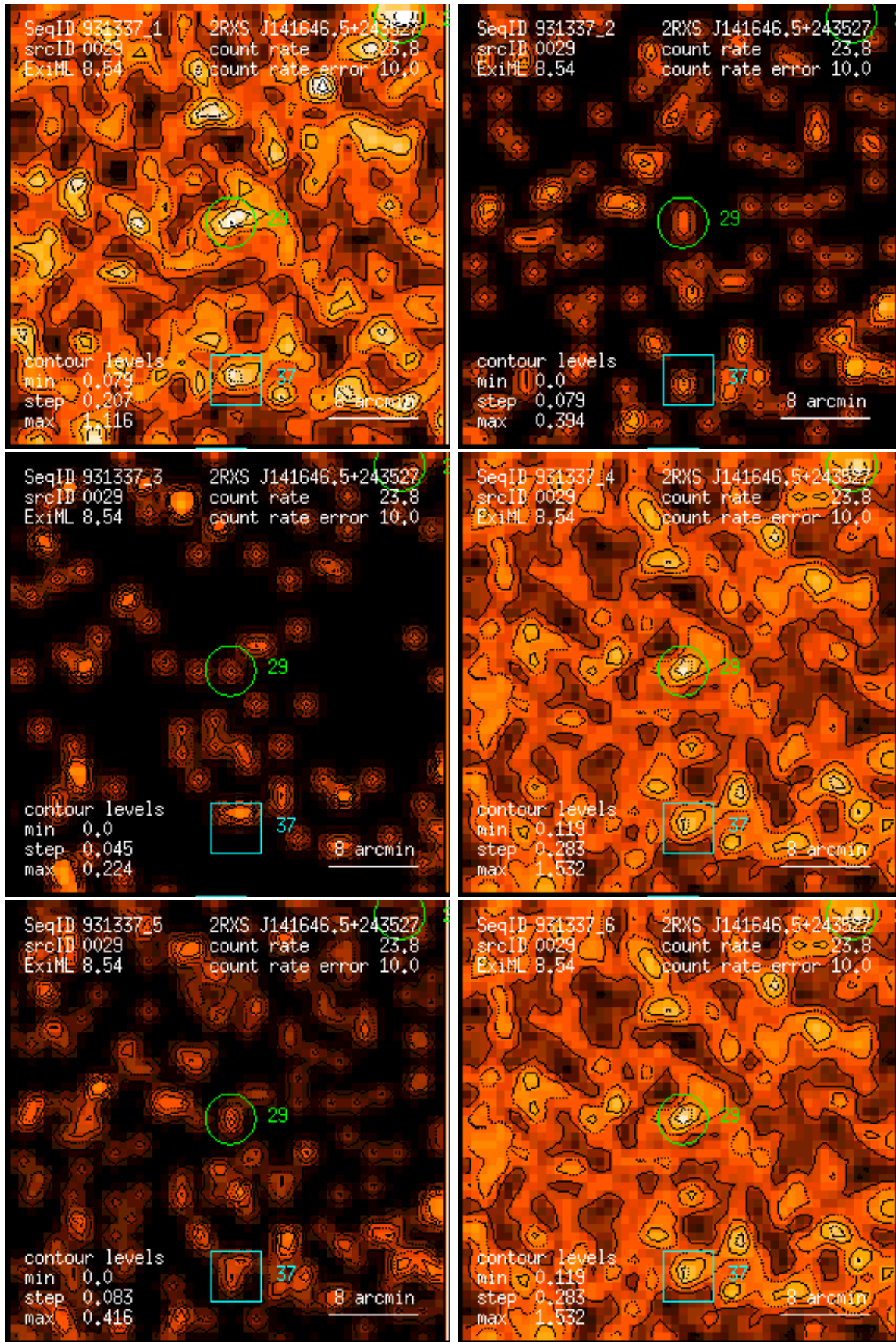
Figure 29: RASS 931337: detection 0029: band rate images, Gaussian filter: (1) PSPC channels 11 – 41, (2) 52 – 90, (3) 91 – 201, (4) 11 – 235, (5) 52 – 201, (6) 11 – 201. Broad band rates in counts/ks. Band rate contour levels in counts/ks/arcmin 2 .
