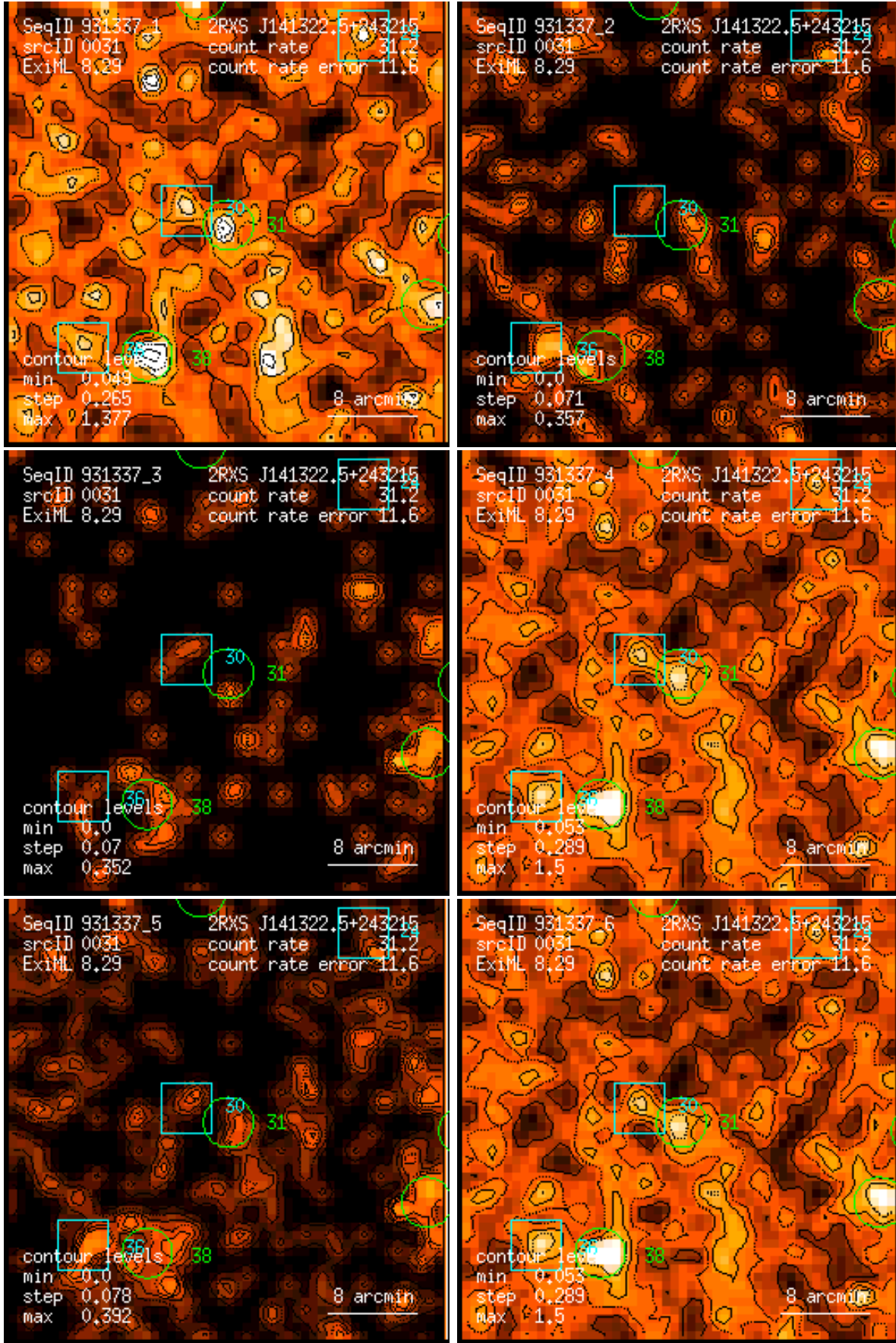
Figure 31: RASS 931337: detection 0031: band rate images, Gaussian filter: (1) PSPC channels 11 – 41, (2) 52 – 90, (3) 91 – 201, (4) 11 – 235, (5) 52 – 201, (6) 11 – 201. Broad band rates in counts/ks. Band rate contour levels in counts/ks/arcmin 2 .
