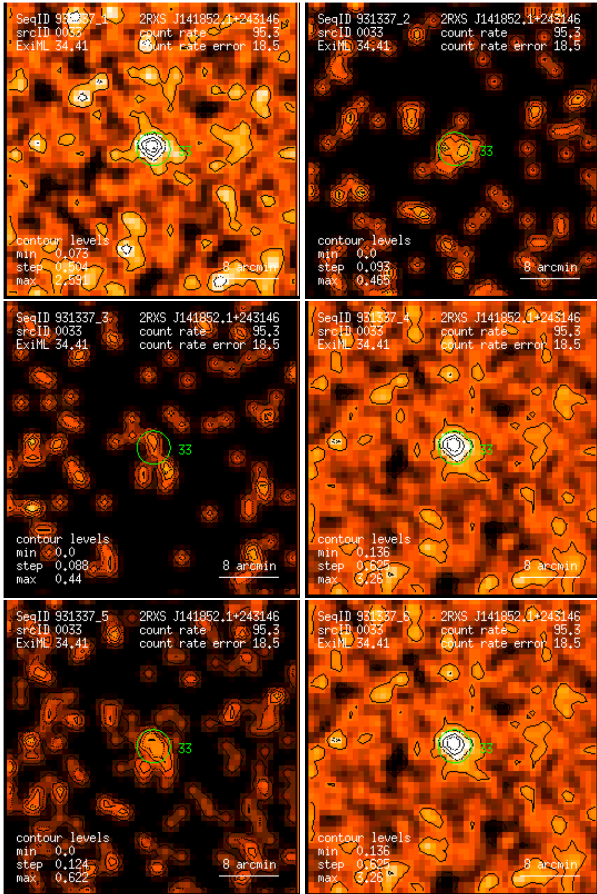
Figure 33: RASS 931337: detection 0033: band rate images, Gaussian filter: (1) PSPC channels 11 – 41, (2) 52 – 90, (3) 91 – 201, (4) 11 – 235, (5) 52 – 201, (6) 11 – 201. Broad band rates in counts/ks. Band rate contour levels in counts/ks/arcmin 2 .
