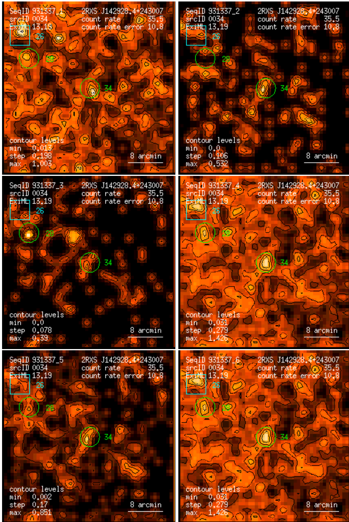
Figure 34: RASS 931337: detection 0034: band rate images, Gaussian filter: (1) PSPC channels 11 – 41, (2) 52 – 90, (3) 91 – 201, (4) 11 – 235, (5) 52 – 201, (6) 11 – 201. Broad band rates in counts/ks. Band rate contour levels in counts/ks/arcmin 2 .
