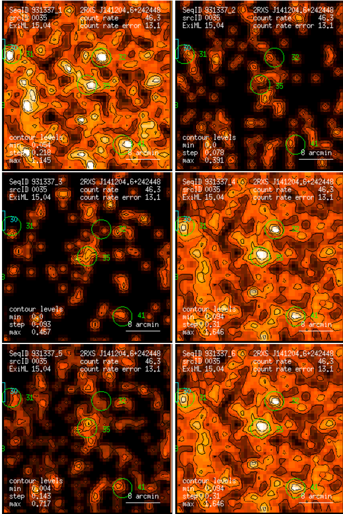
Figure 35: RASS 931337: detection 0035: band rate images, Gaussian filter: (1) PSPC channels 11 – 41, (2) 52 – 90, (3) 91 – 201, (4) 11 – 235, (5) 52 – 201, (6) 11 – 201. Broad band rates in counts/ks. Band rate contour levels in counts/ks/arcmin 2 .
