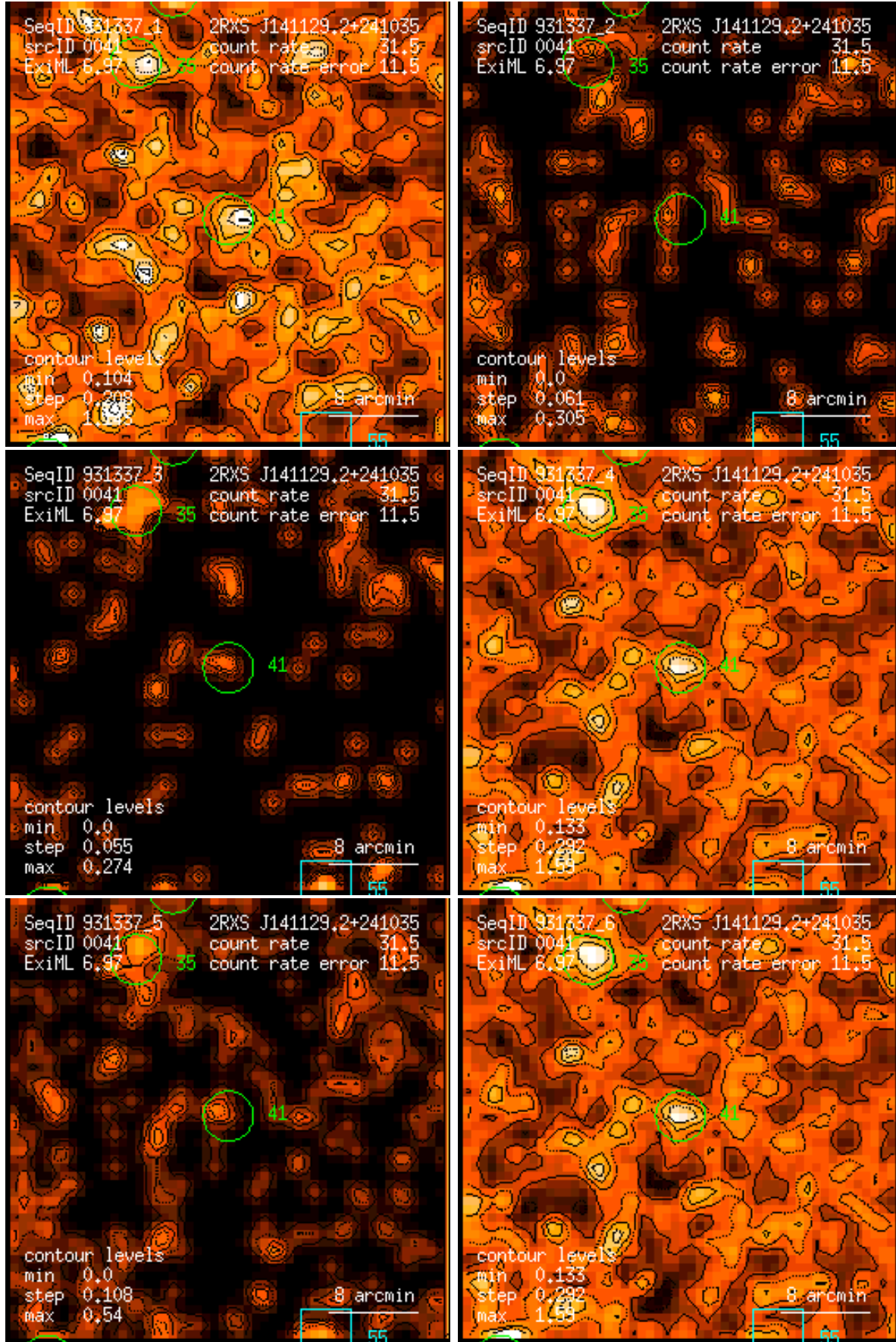
Figure 41: RASS 931337: detection 0041: band rate images, Gaussian filter: (1) PSPC channels 11 – 41, (2) 52 – 90, (3) 91 – 201, (4) 11 – 235, (5) 52 – 201, (6) 11 – 201. Broad band rates in counts/ks. Band rate contour levels in counts/ks/arcmin 2 .
