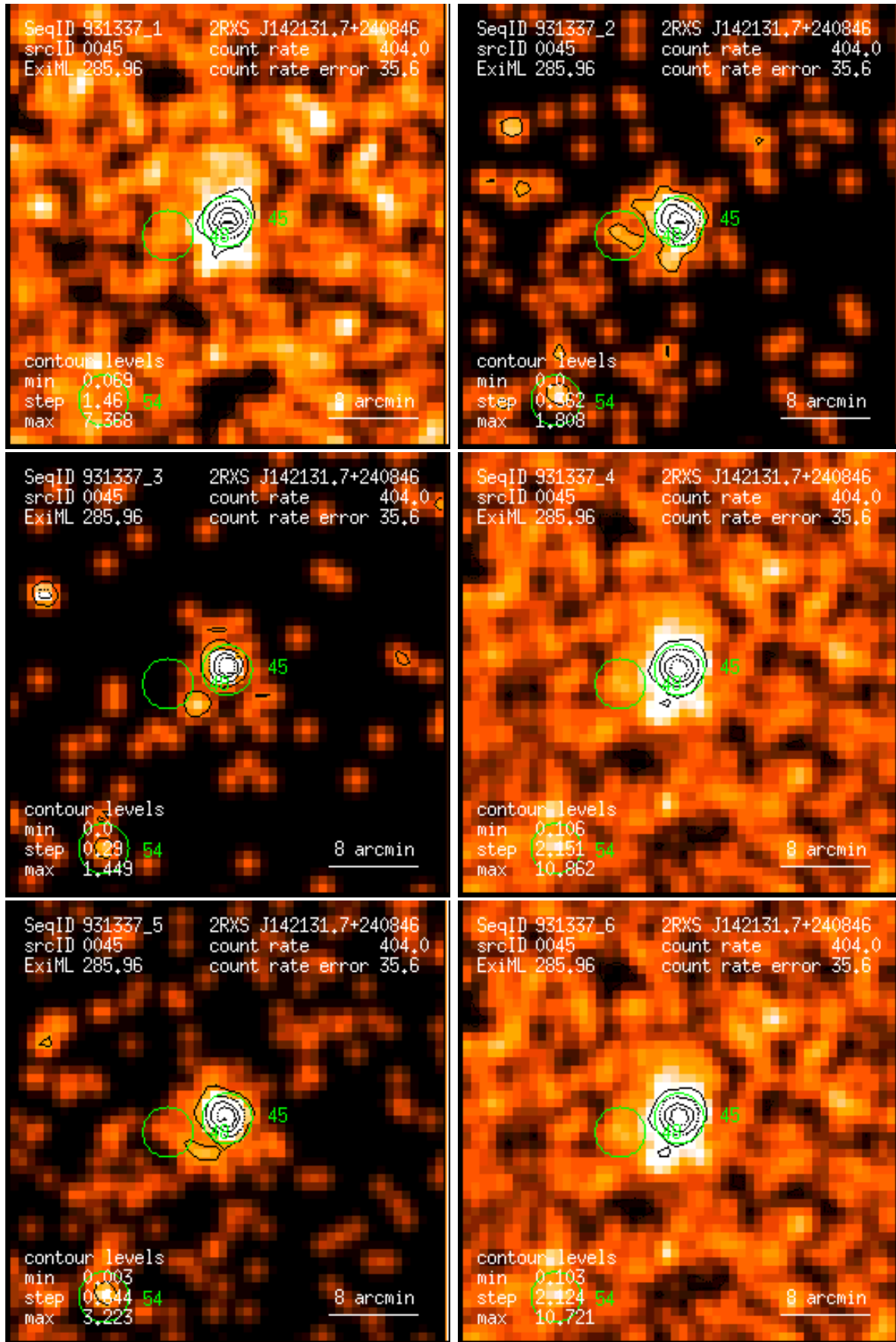
Figure 45: RASS 931337: detection 0045: band rate images, Gaussian filter: (1) PSPC channels 11 – 41, (2) 52 – 90, (3) 91 – 201, (4) 11 – 235, (5) 52 – 201, (6) 11 – 201. Broad band rates in counts/ks. Band rate contour levels in counts/ks/arcmin 2 .
