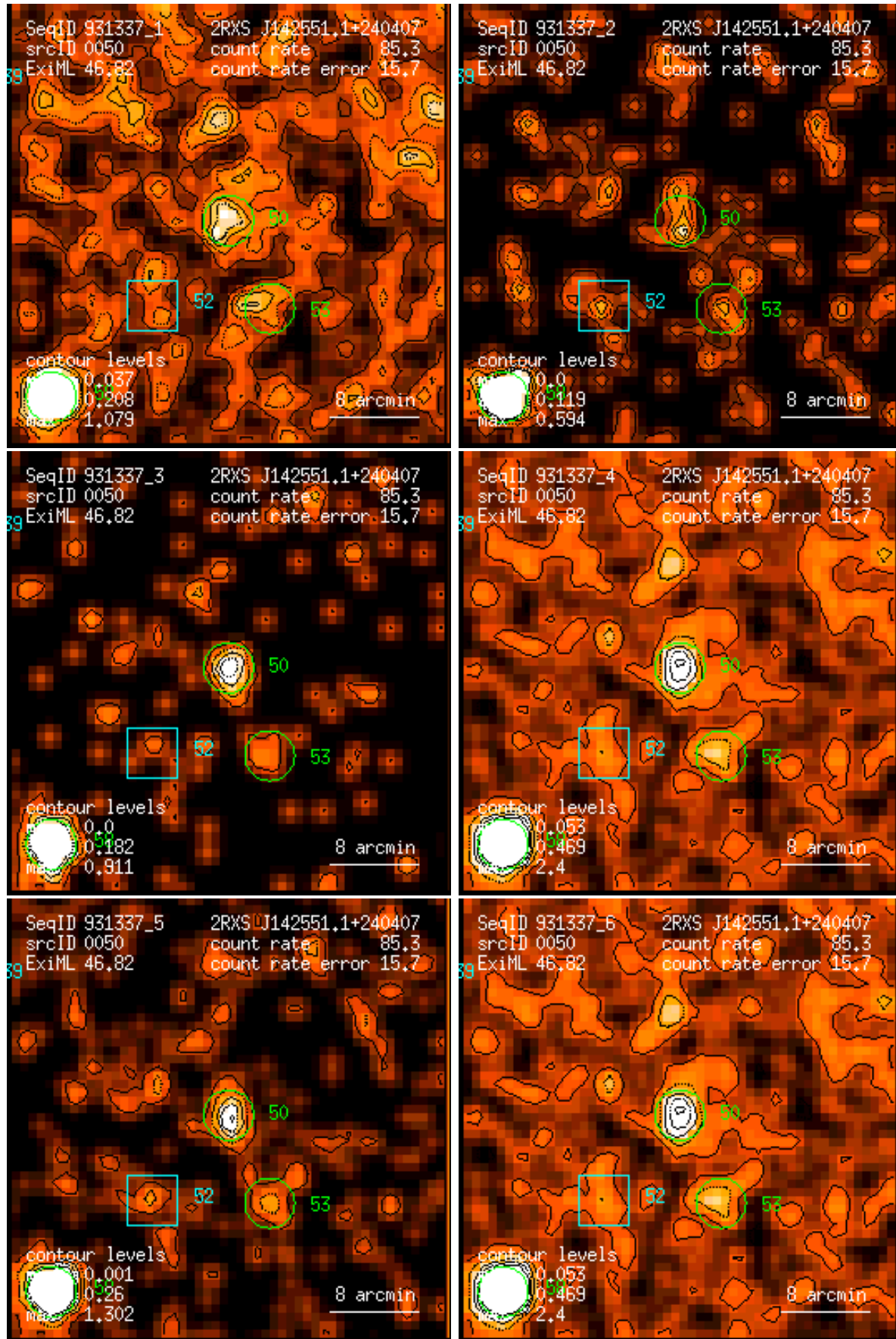
Figure 50: RASS 931337: detection 0050: band rate images, Gaussian filter: (1) PSPC channels 11 – 41, (2) 52 – 90, (3) 91 – 201, (4) 11 – 235, (5) 52 – 201, (6) 11 – 201. Broad band rates in counts/ks. Band rate contour levels in counts/ks/arcmin 2 .
