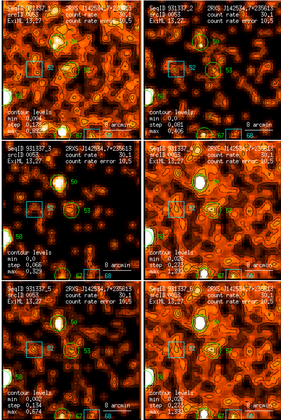
Figure 53: RASS 931337: detection 0053: band rate images, Gaussian filter: (1) PSPC channels 11 – 41, (2) 52 – 90, (3) 91 – 201, (4) 11 – 235, (5) 52 – 201, (6) 11 – 201. Broad band rates in counts/ks. Band rate contour levels in counts/ks/arcmin 2 .
