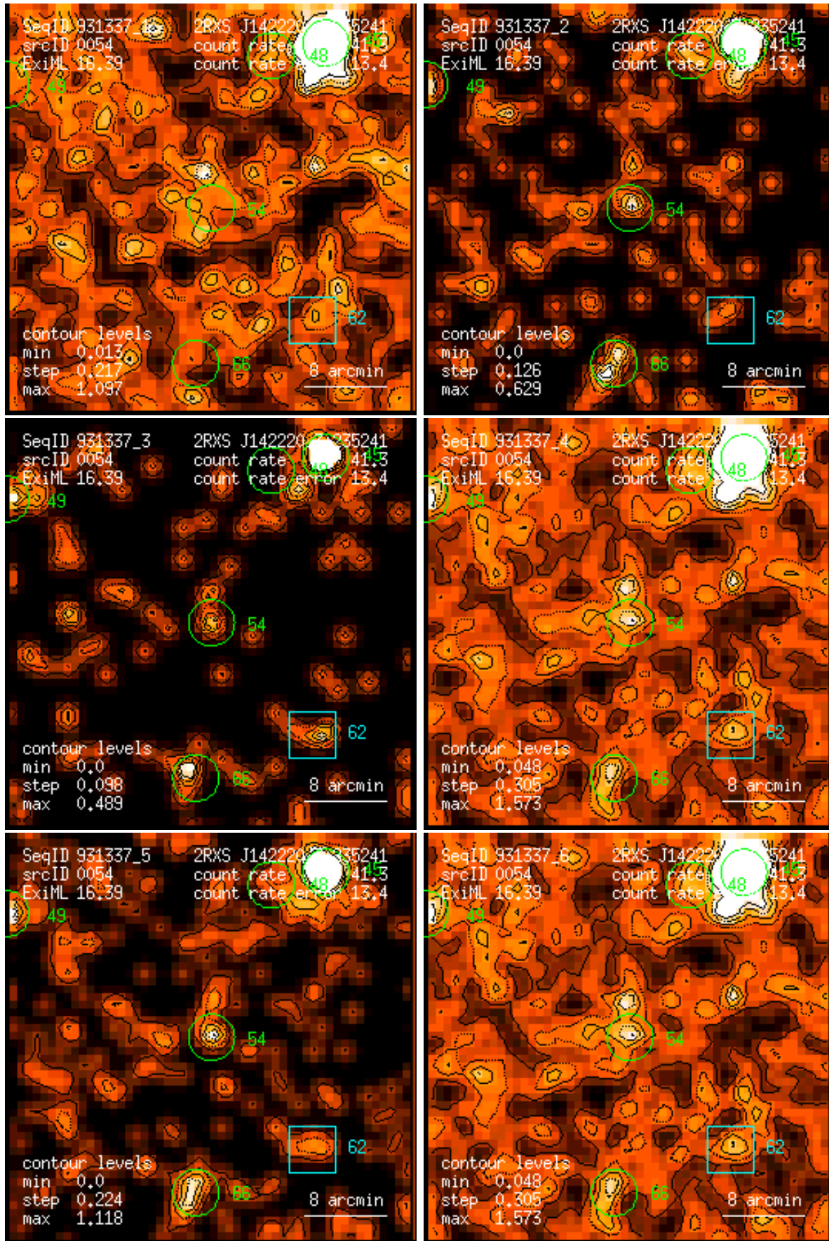
Figure 54: RASS 931337: detection 0054: band rate images, Gaussian filter: (1) PSPC channels 11 – 41, (2) 52 – 90, (3) 91 – 201, (4) 11 – 235, (5) 52 – 201, (6) 11 – 201. Broad band rates in counts/ks. Band rate contour levels in counts/ks/arcmin 2 .
