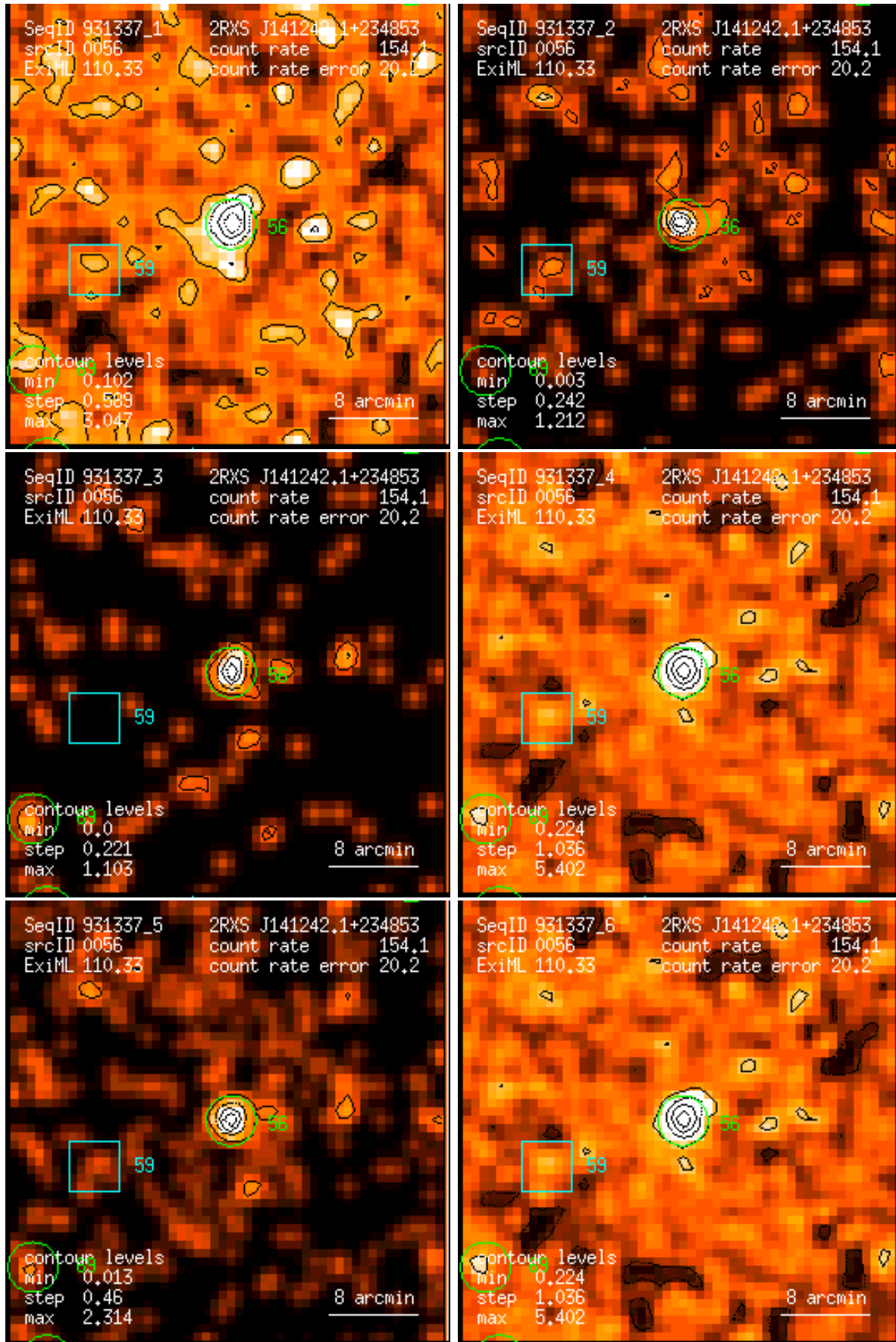
Figure 56: RASS 931337: detection 0056: band rate images, Gaussian filter: (1) PSPC channels 11 – 41, (2) 52 – 90, (3) 91 – 201, (4) 11 – 235, (5) 52 – 201, (6) 11 – 201. Broad band rates in counts/ks. Band rate contour levels in counts/ks/arcmin 2 .
