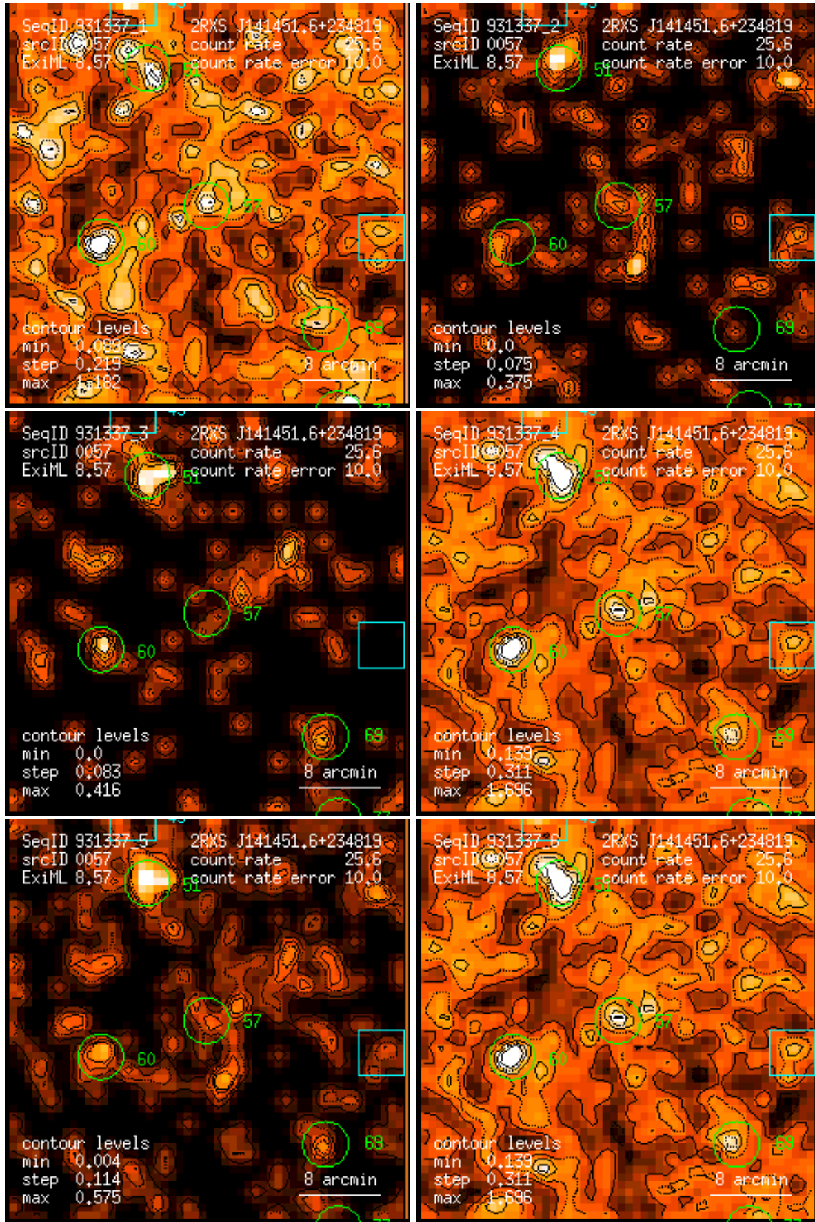
Figure 57: RASS 931337: detection 0057: band rate images, Gaussian filter: (1) PSPC channels 11 – 41, (2) 52 – 90, (3) 91 – 201, (4) 11 – 235, (5) 52 – 201, (6) 11 – 201. Broad band rates in counts/ks. Band rate contour levels in counts/ks/arcmin 2 .
