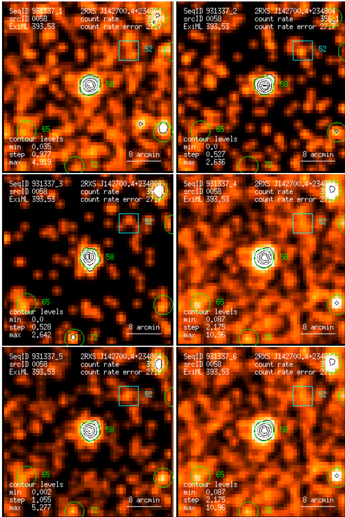
Figure 58: RASS 931337: detection 0058: band rate images, Gaussian filter: (1) PSPC channels 11 – 41, (2) 52 – 90, (3) 91 – 201, (4) 11 – 235, (5) 52 – 201, (6) 11 – 201. Broad band rates in counts/ks. Band rate contour levels in counts/ks/arcmin 2 .
