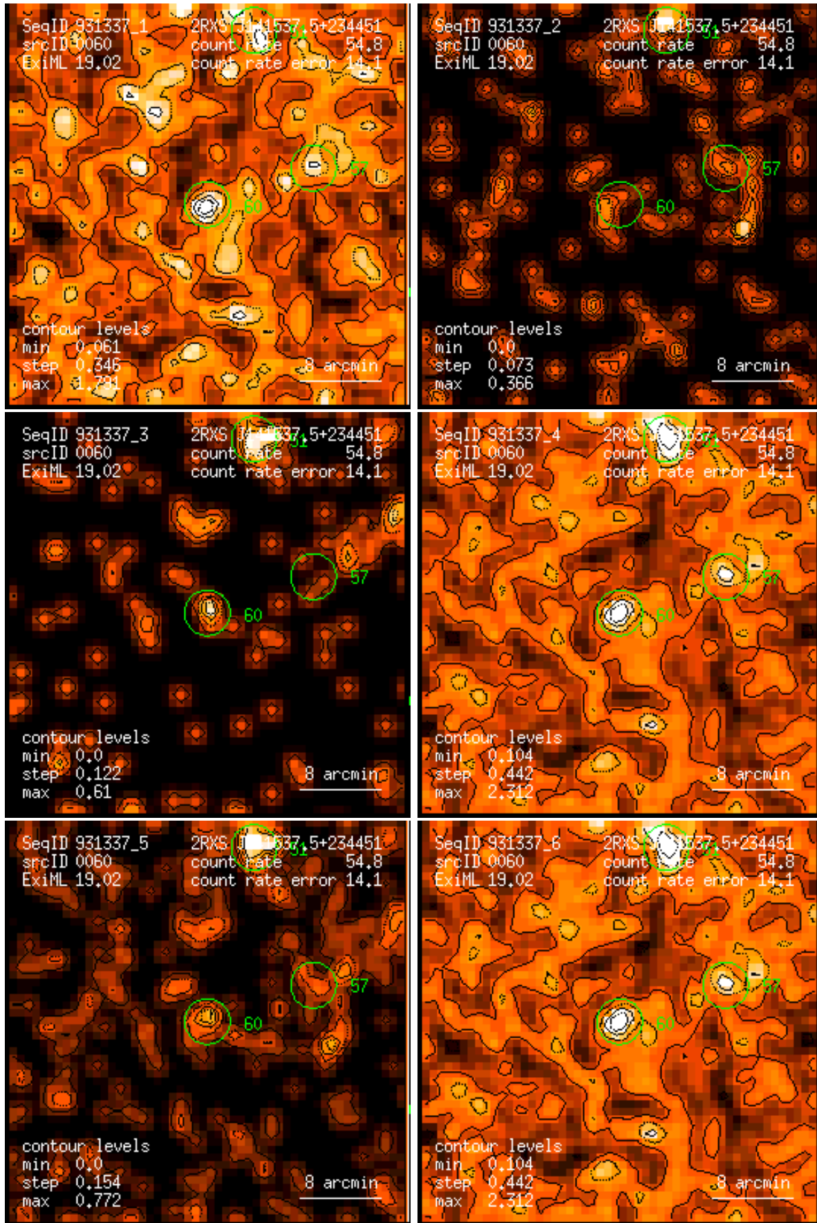
Figure 60: RASS 931337: detection 0060: band rate images, Gaussian filter: (1) PSPC channels 11 – 41, (2) 52 – 90, (3) 91 – 201, (4) 11 – 235, (5) 52 – 201, (6) 11 – 201. Broad band rates in counts/ks. Band rate contour levels in counts/ks/arcmin 2 .
