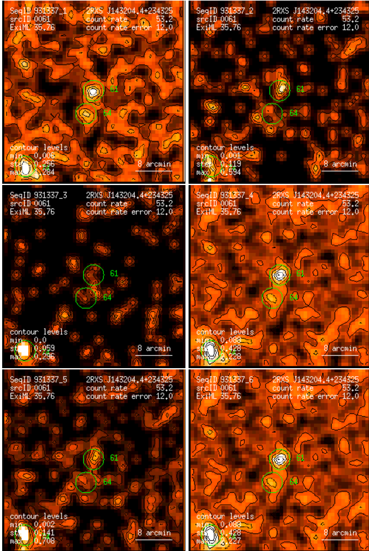
Figure 61: RASS 931337: detection 0061: band rate images, Gaussian filter: (1) PSPC channels 11 – 41, (2) 52 – 90, (3) 91 – 201, (4) 11 – 235, (5) 52 – 201, (6) 11 – 201. Broad band rates in counts/ks. Band rate contour levels in counts/ks/arcmin 2 .
