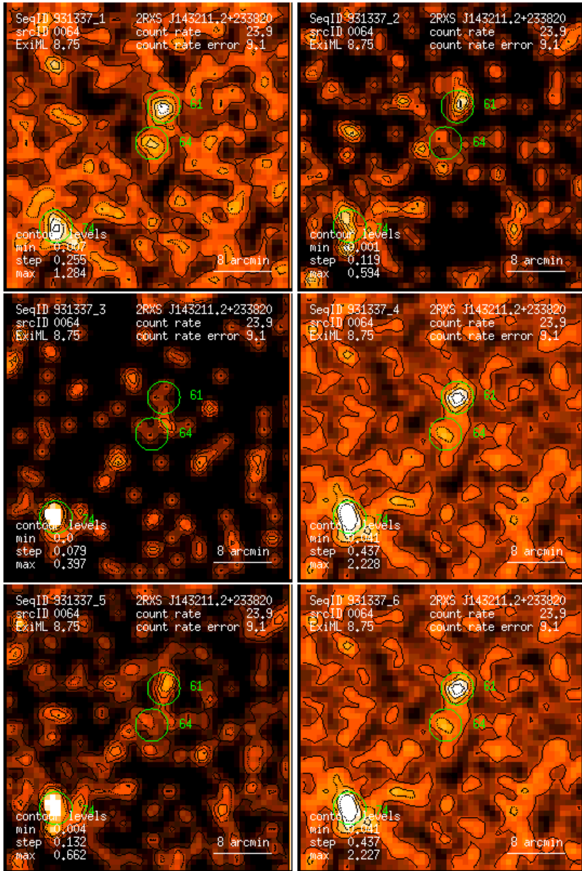
Figure 64: RASS 931337: detection 0064: band rate images, Gaussian filter: (1) PSPC channels 11 – 41, (2) 52 – 90, (3) 91 – 201, (4) 11 – 235, (5) 52 – 201, (6) 11 – 201. Broad band rates in counts/ks. Band rate contour levels in counts/ks/arcmin 2 .
