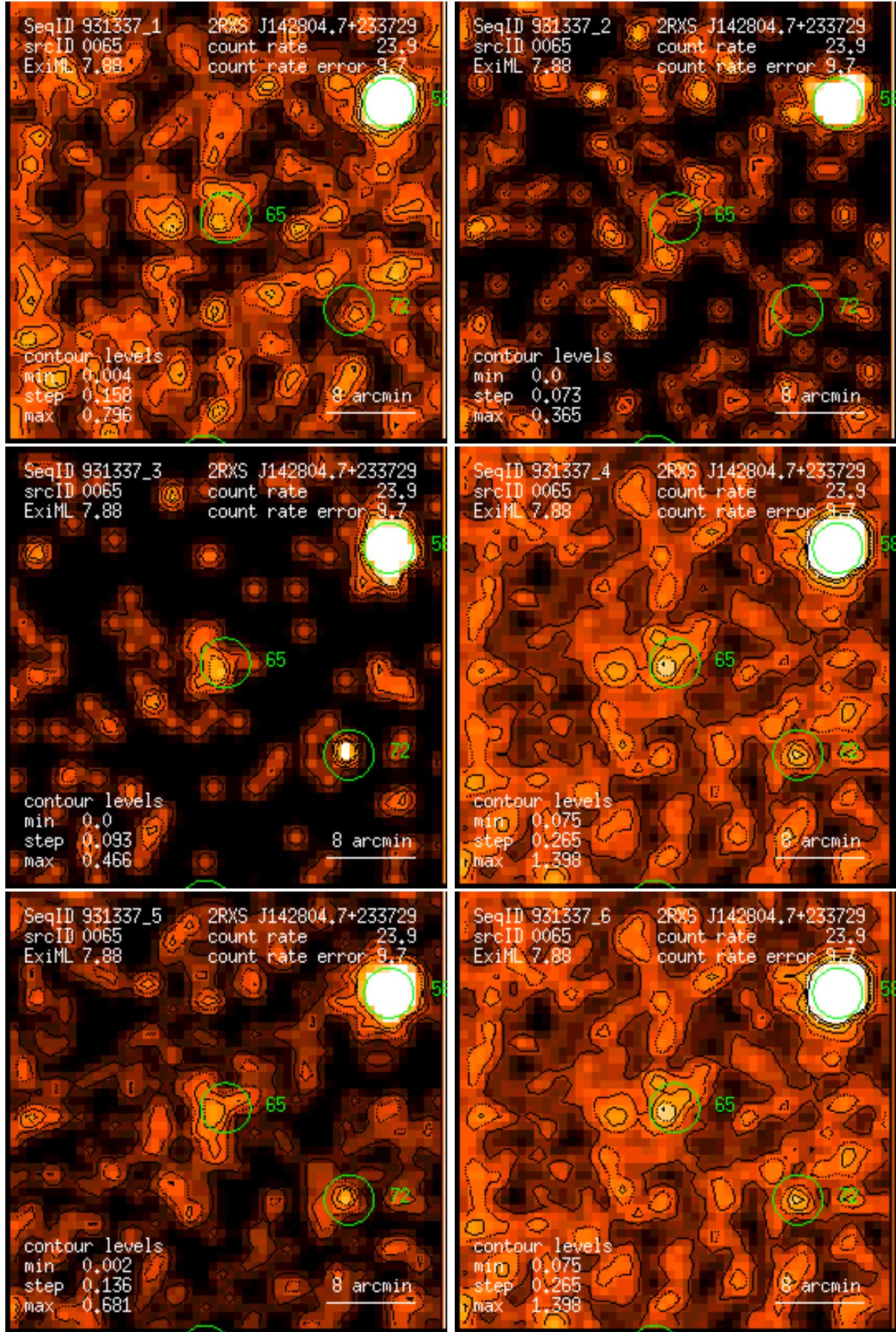
Figure 65: RASS 931337: detection 0065: band rate images, Gaussian filter: (1) PSPC channels 11 – 41, (2) 52 – 90, (3) 91 – 201, (4) 11 – 235, (5) 52 – 201, (6) 11 – 201. Broad band rates in counts/ks. Band rate contour levels in counts/ks/arcmin 2 .
