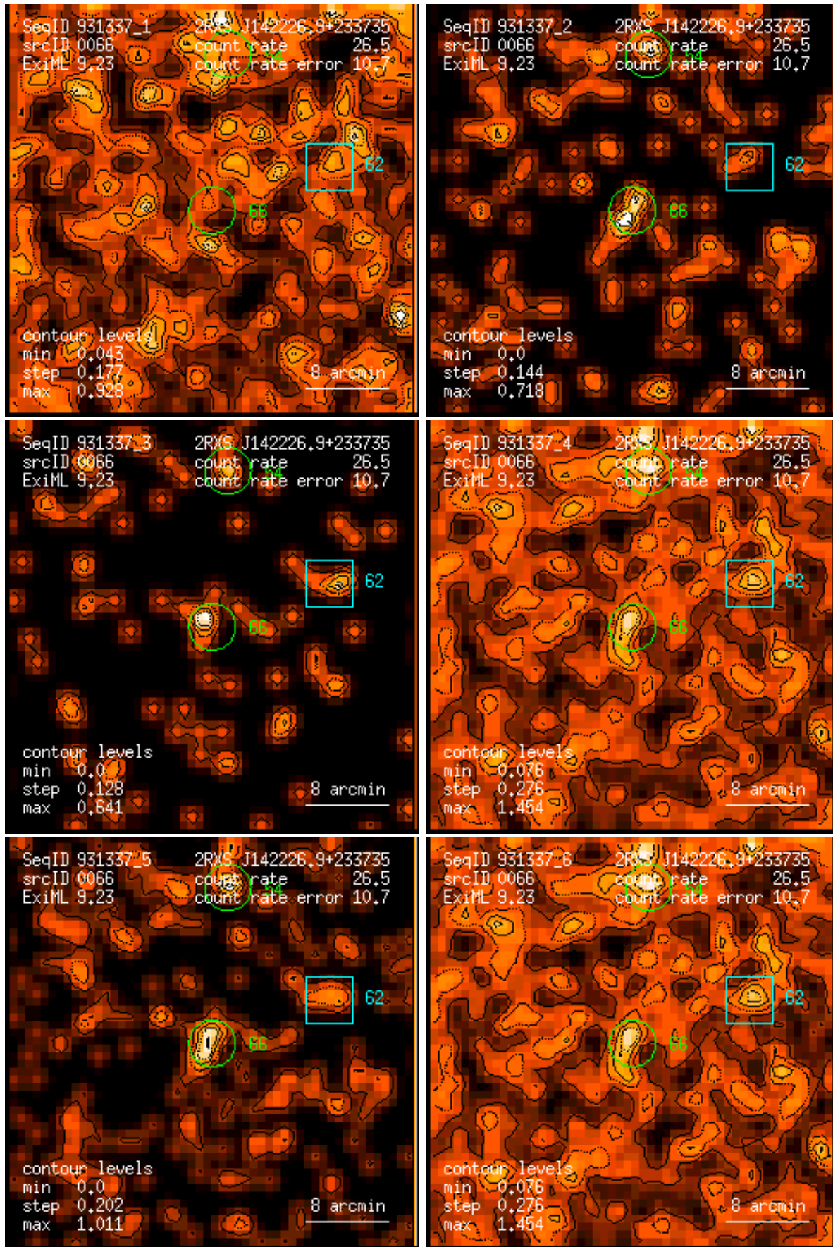
Figure 66: RASS 931337: detection 0066: band rate images, Gaussian filter: (1) PSPC channels 11 – 41, (2) 52 – 90, (3) 91 – 201, (4) 11 – 235, (5) 52 – 201, (6) 11 – 201. Broad band rates in counts/ks. Band rate contour levels in counts/ks/arcmin 2 .
