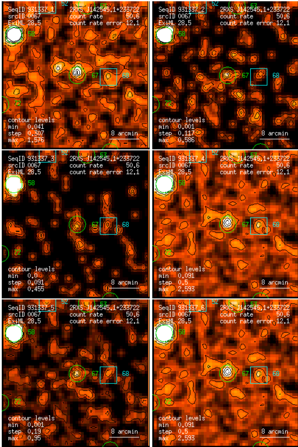
Figure 67: RASS 931337: detection 0067: band rate images, Gaussian filter: (1) PSPC channels 11 – 41, (2) 52 – 90, (3) 91 – 201, (4) 11 – 235, (5) 52 – 201, (6) 11 – 201. Broad band rates in counts/ks. Band rate contour levels in counts/ks/arcmin 2 .
