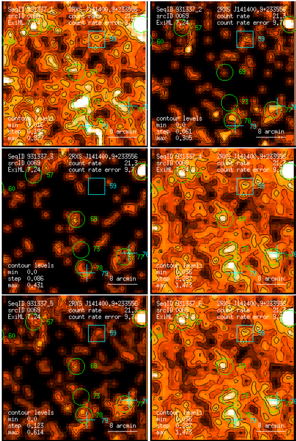
Figure 69: RASS 931337: detection 0069: band rate images, Gaussian filter: (1) PSPC channels 11 – 41, (2) 52 – 90, (3) 91 – 201, (4) 11 – 235, (5) 52 – 201, (6) 11 – 201. Broad band rates in counts/ks. Band rate contour levels in counts/ks/arcmin 2 .
