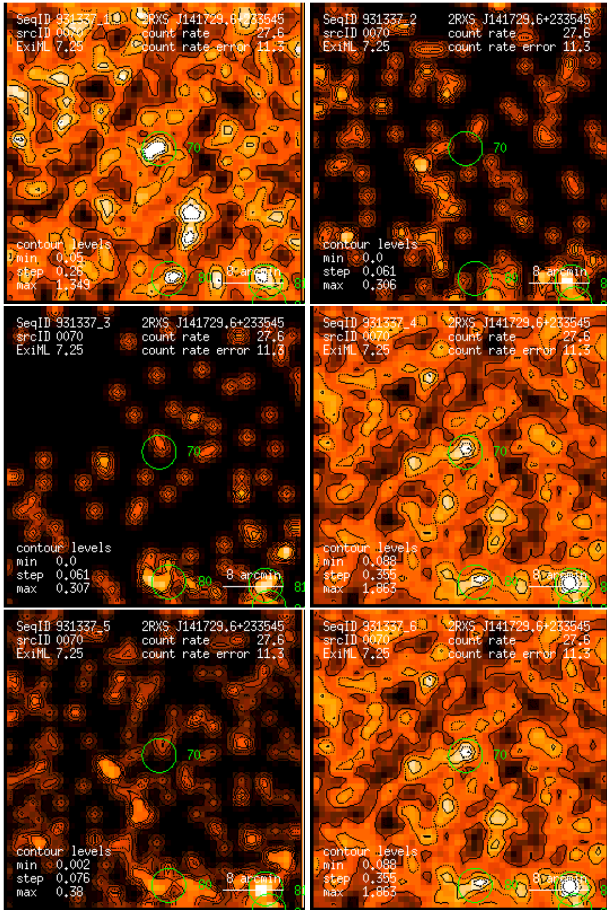
Figure 70: RASS 931337: detection 0070: band rate images, Gaussian filter: (1) PSPC channels 11 – 41, (2) 52 – 90, (3) 91 – 201, (4) 11 – 235, (5) 52 – 201, (6) 11 – 201. Broad band rates in counts/ks. Band rate contour levels in counts/ks/arcmin 2 .
