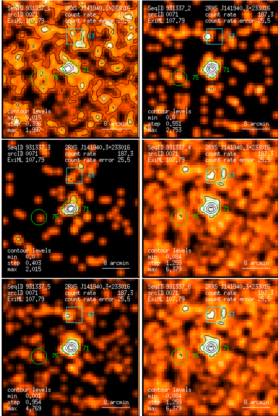
Figure 71: RASS 931337: detection 0071: band rate images, Gaussian filter: (1) PSPC channels 11 – 41, (2) 52 – 90, (3) 91 – 201, (4) 11 – 235, (5) 52 – 201, (6) 11 – 201. Broad band rates in counts/ks. Band rate contour levels in counts/ks/arcmin 2 .
