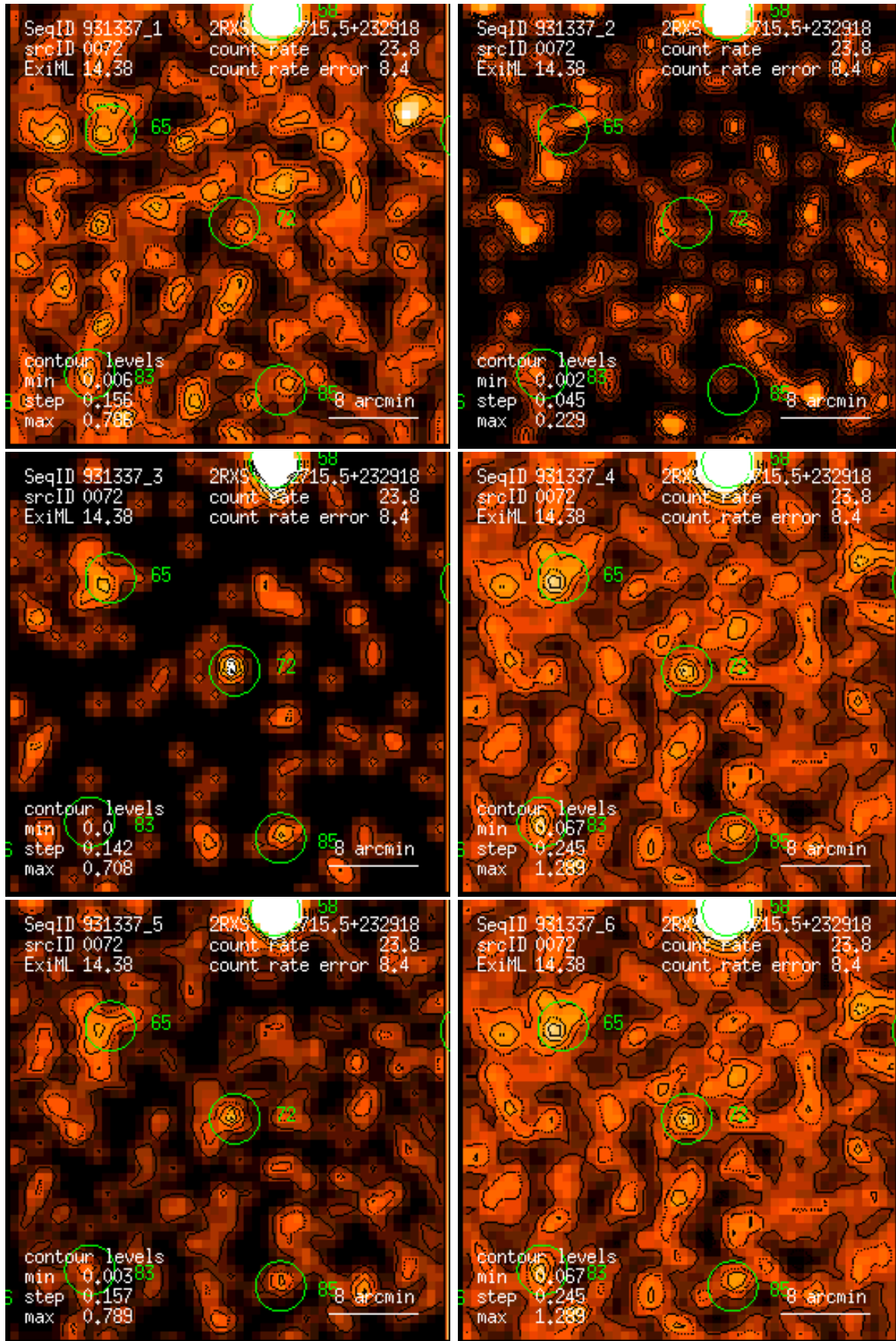
Figure 72: RASS 931337: detection 0072: band rate images, Gaussian filter: (1) PSPC channels 11 – 41, (2) 52 – 90, (3) 91 – 201, (4) 11 – 235, (5) 52 – 201, (6) 11 – 201. Broad band rates in counts/ks. Band rate contour levels in counts/ks/arcmin 2 .
