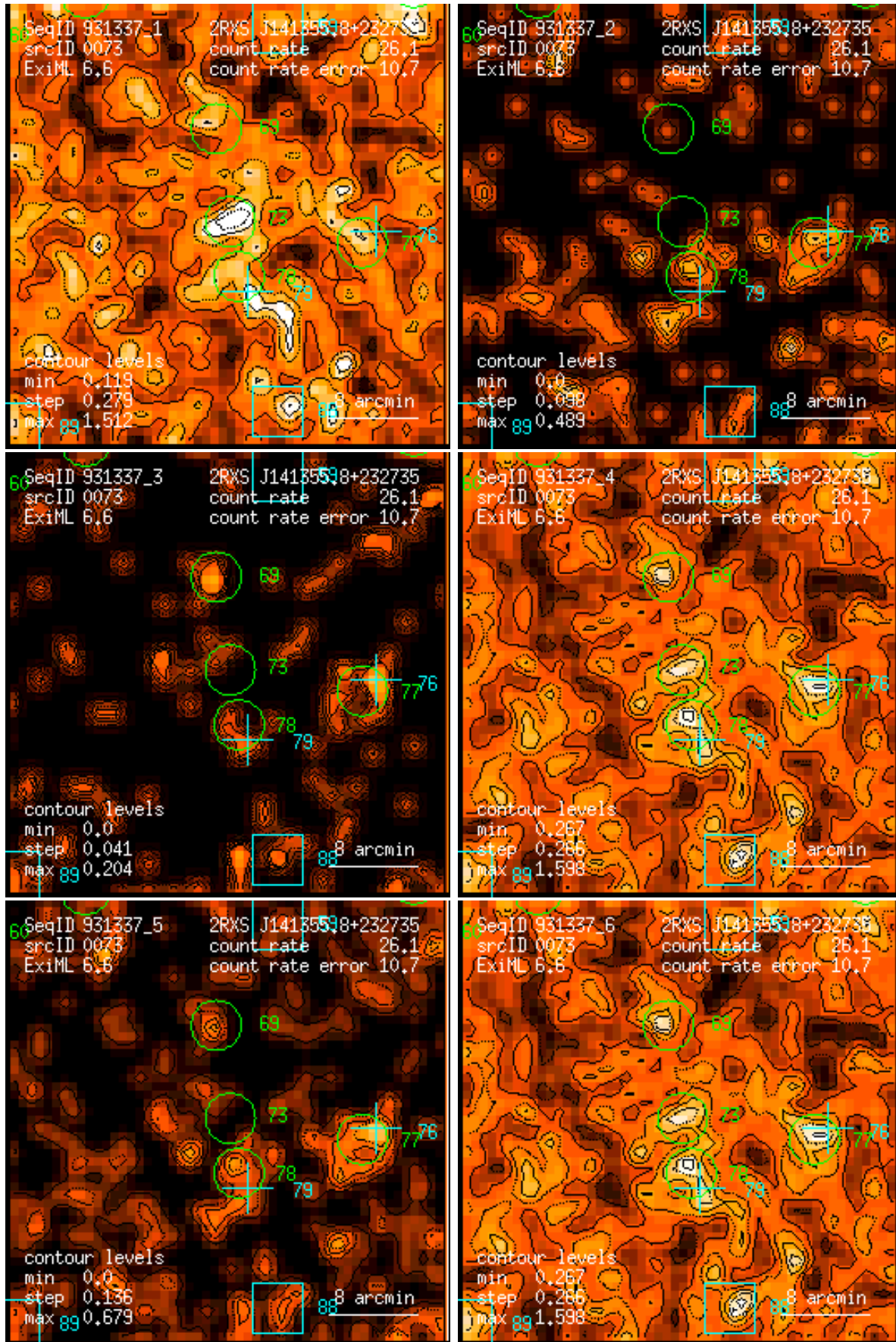
Figure 73: RASS 931337: detection 0073: band rate images, Gaussian filter: (1) PSPC channels 11 – 41, (2) 52 – 90, (3) 91 – 201, (4) 11 – 235, (5) 52 – 201, (6) 11 – 201. Broad band rates in counts/ks. Band rate contour levels in counts/ks/arcmin 2 .
