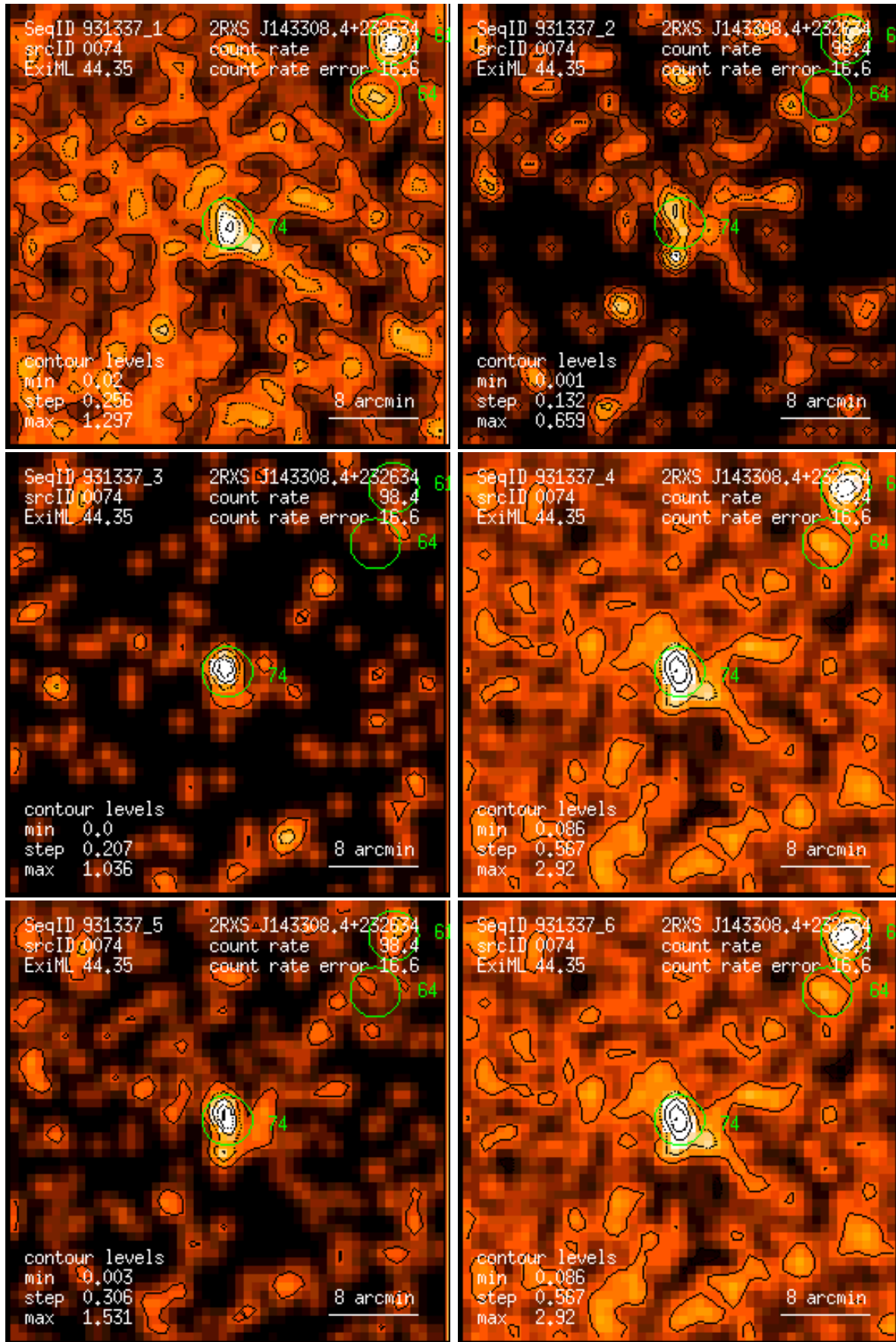
Figure 74: RASS 931337: detection 0074: band rate images, Gaussian filter: (1) PSPC channels 11 – 41, (2) 52 – 90, (3) 91 – 201, (4) 11 – 235, (5) 52 – 201, (6) 11 – 201. Broad band rates in counts/ks. Band rate contour levels in counts/ks/arcmin 2 .
